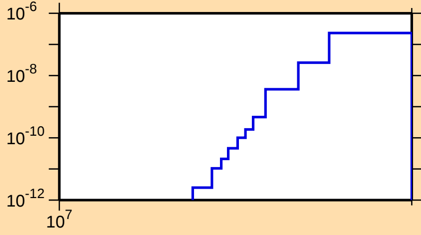
\sigma vs. E for ^{121}\text{I} (mt 45)
