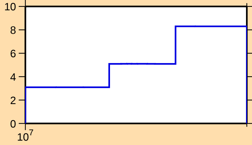
\Delta\sigma/\sigma vs. E for ^{121}\text{I}(n,\text{tot.})
