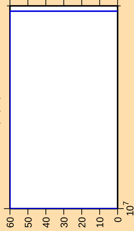
\Delta\sigma/\sigma vs. E for ^{121}\text{I}(\text{n},\text{pd})
