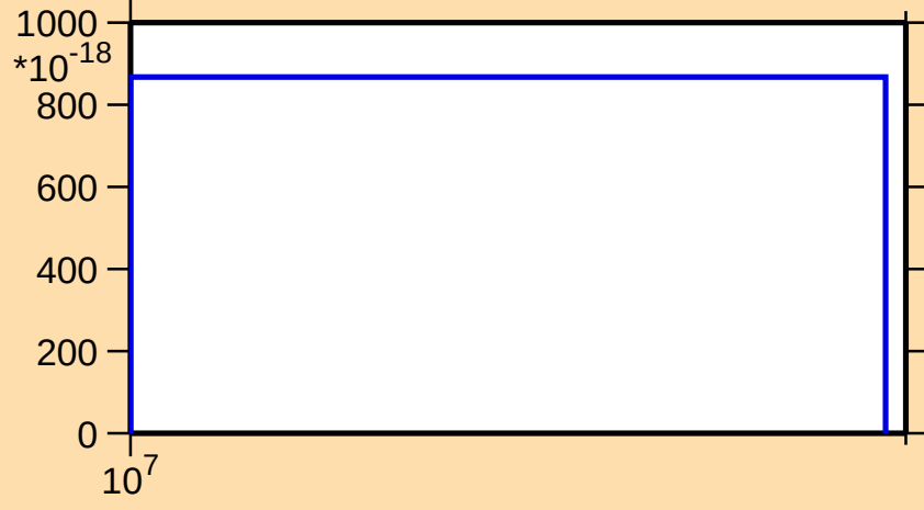
\sigma vs. E for ^{121}\text{I} (mt 34)
