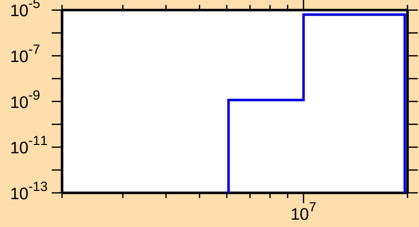
\sigma vs. E for ^{121}\text{I}(n,p\alpha)
