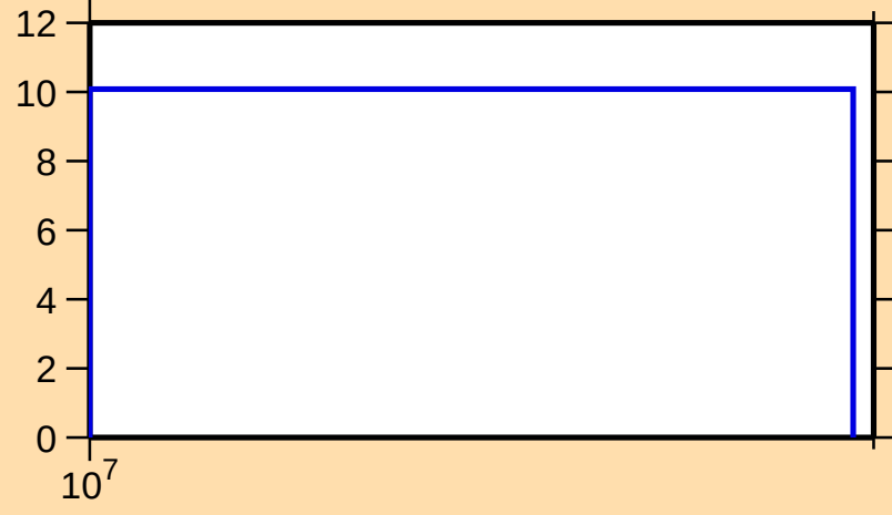
\Delta\sigma/\sigma vs. E for ^{121}\text{I}(n,\text{el.})
