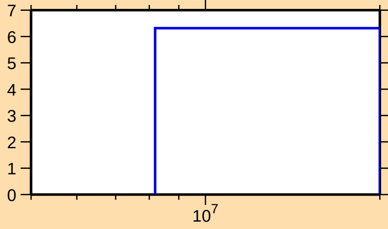
\Delta\sigma/\sigma vs. E for ^{121}\text{I}(n,\text{nonel.})
