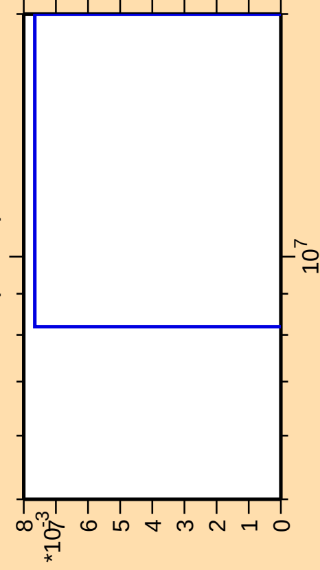
\Delta\sigma/\sigma vs. E for ^{121}\text{I}(\text{mt 34})
