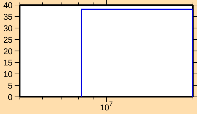
\Delta\sigma/\sigma vs. E for ^{121}\text{I}(n,\text{inel.})
