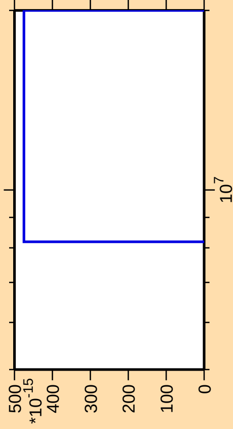
\Delta\sigma/\sigma vs. E for ^{121}\text{I}(\text{mt 11})
