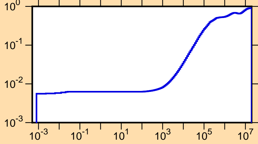
\mu vs. E for ^{122}\text{I}(\text{mt251})
