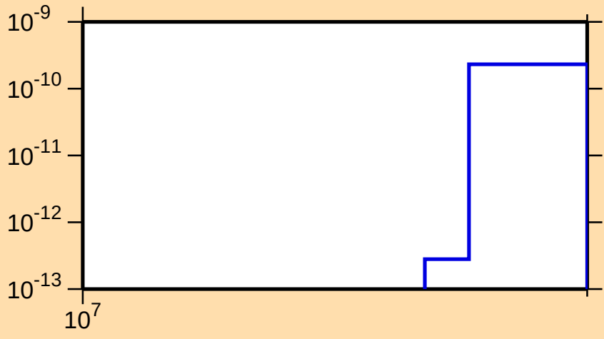
\sigma vs. E for ^{122}\text{I}(n,\text{pt})
