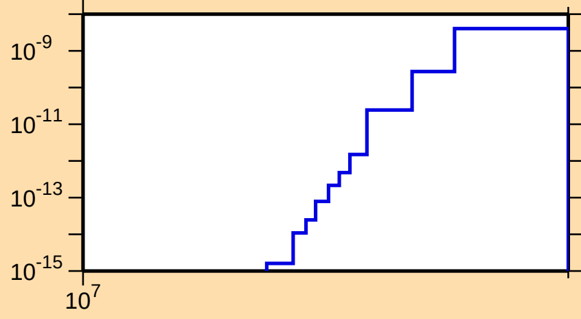
\sigma vs. E for ^{122}\text{I} (mt 45)
