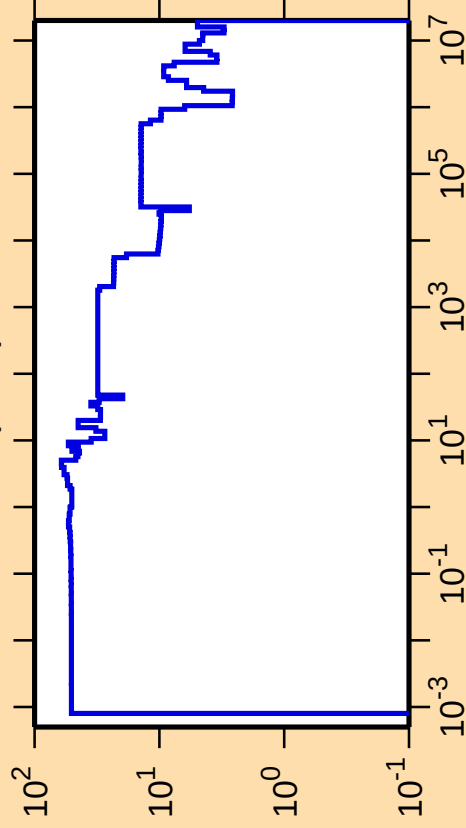
\Delta\sigma/\sigma vs. E for ^{122}\text{I}(n,\text{el.})
