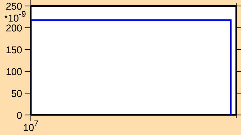
\sigma vs. E for ^{122}\text{I}(n,2n\alpha)
