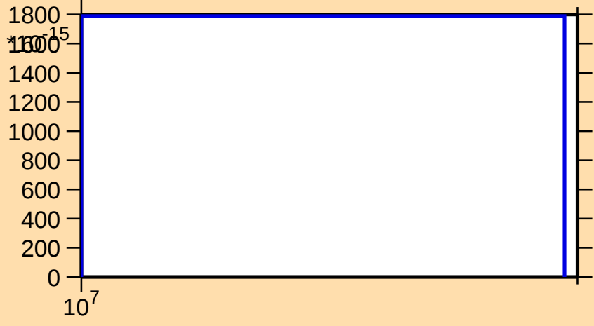
\sigma vs. E for ^{122}\text{I}(\text{n},\text{pt})
