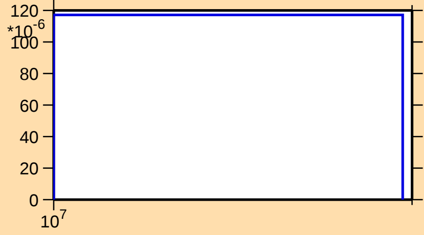
\sigma vs. E for ^{122}\text{I}(n,2np)
