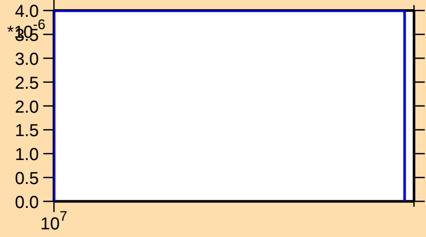
\sigma vs. E for ^{122}\text{I}(\text{n},\text{nd})
