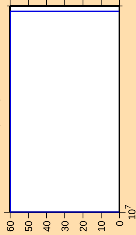
\Delta\sigma/\sigma vs. E for ^{122}\text{I}(\text{n},\text{nd})
