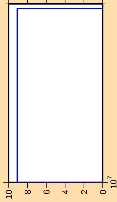
\Delta\sigma/\sigma vs. E for ^{122}\text{I}(\text{n},\text{pt})
