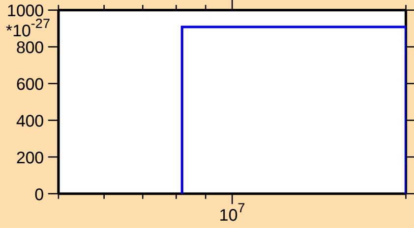
\sigma vs. E for ^{129}\text{I}(\text{mt 11})
