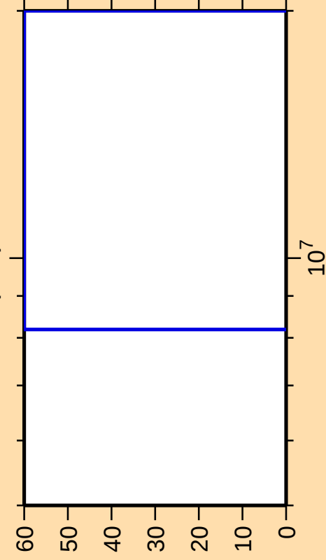
\Delta\sigma/\sigma vs. E for ^{129}\text{I}(n,\alpha)
