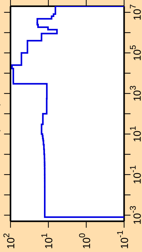
\Delta\sigma/\sigma vs. E for ^{129}\text{I}(\text{n,el.})
