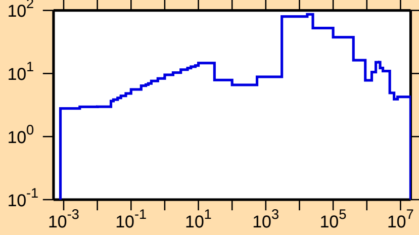
\Delta\sigma/\sigma vs. E for ^{129}\text{I}(\text{n,tot.})
