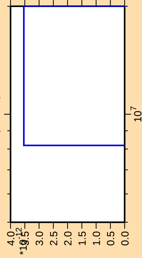
\Delta\sigma/\sigma vs. E for ^{129}\text{I}(\text{mt 11})
