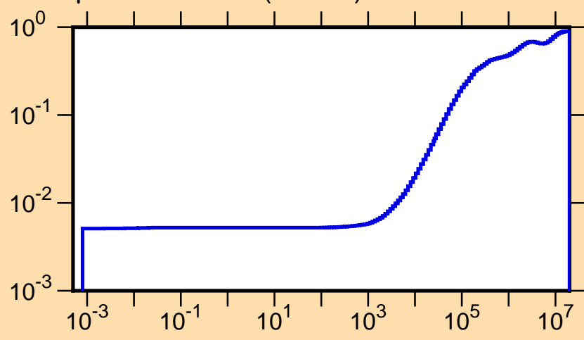
\mu vs. E for ^{132}\text{I}(\text{mt251})
