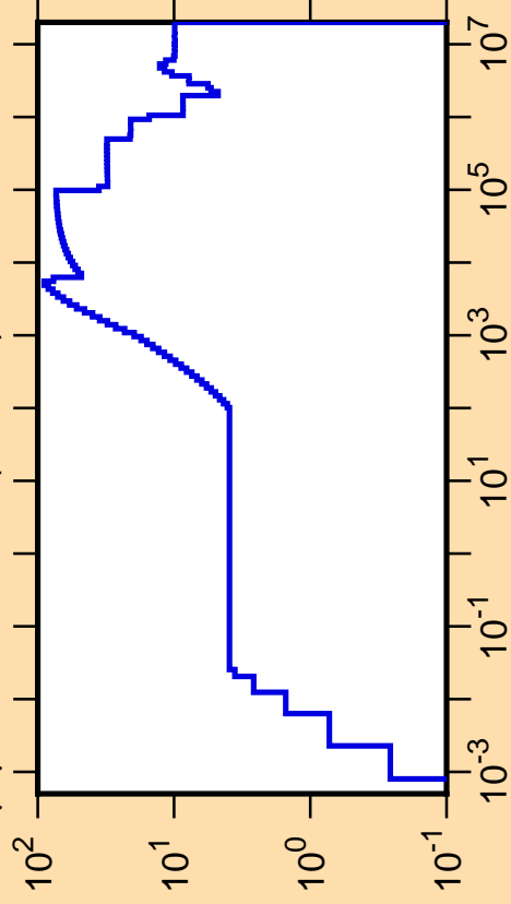
\Delta\mu/\mu vs. E for ^{132}\text{I}(\text{mt251})
