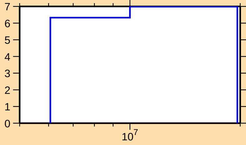
\Delta\sigma/\sigma vs. E for ^{132}\text{I}(n,\text{tot.})
