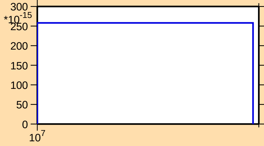
\sigma vs. E for ^{132}\text{I}(n,\text{He3})
