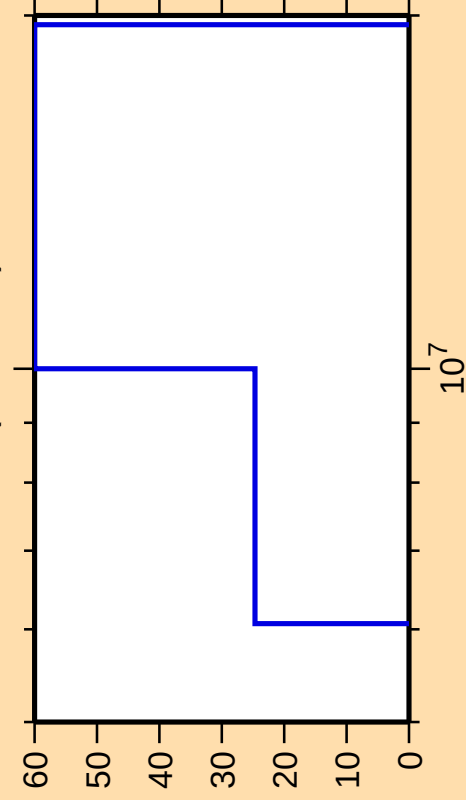
\Delta\sigma/\sigma vs. E for ^{132}\text{I}(n,n\text{cont.})
