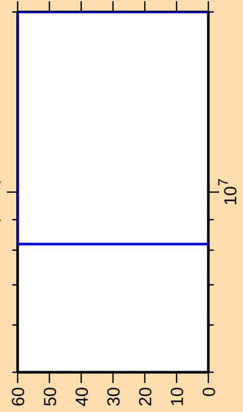
\Delta\sigma/\sigma vs. E for ^{132}\text{I}(n,nt)
