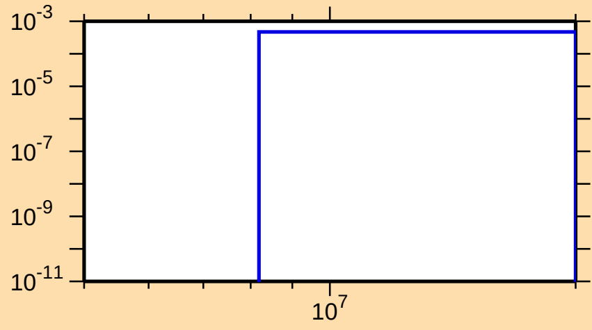
\sigma vs. E for ^{132}\text{I}(n,np)
