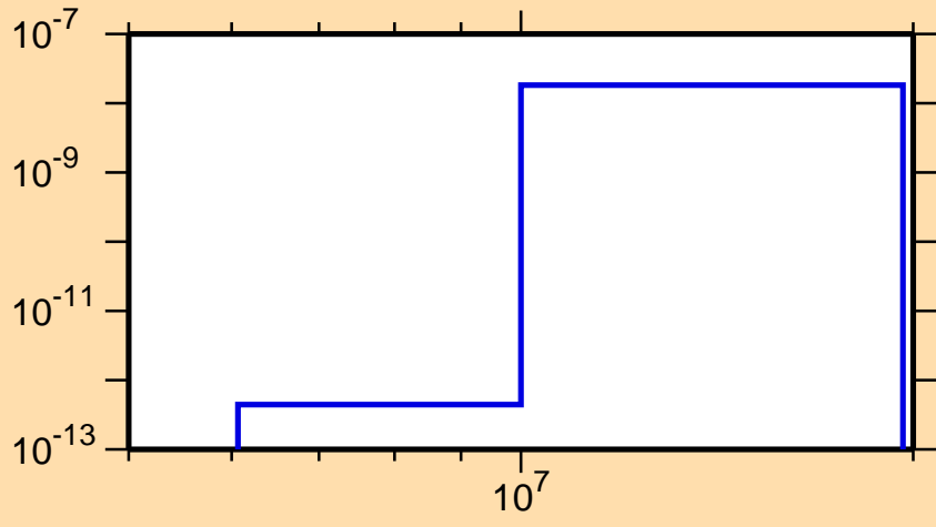
\sigma vs. E for ^{177}\text{Ir}(\text{mt117})
