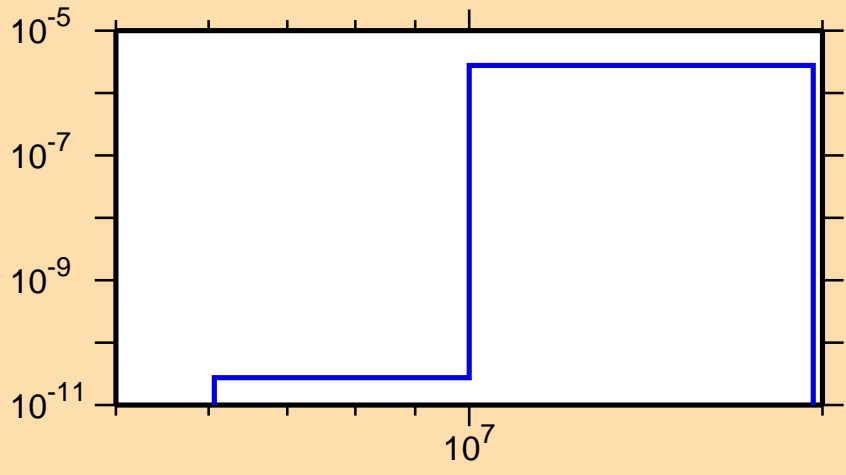
\sigma vs. E for ^{177}\text{Ir}(n,\text{He}3)
