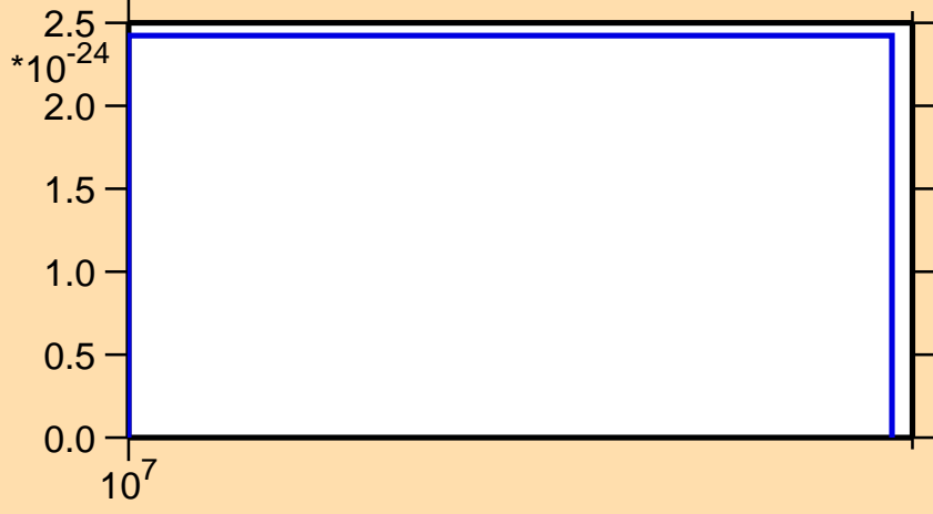
\sigma vs. E for ^{177}\text{Ir}(\text{mt } 42)
