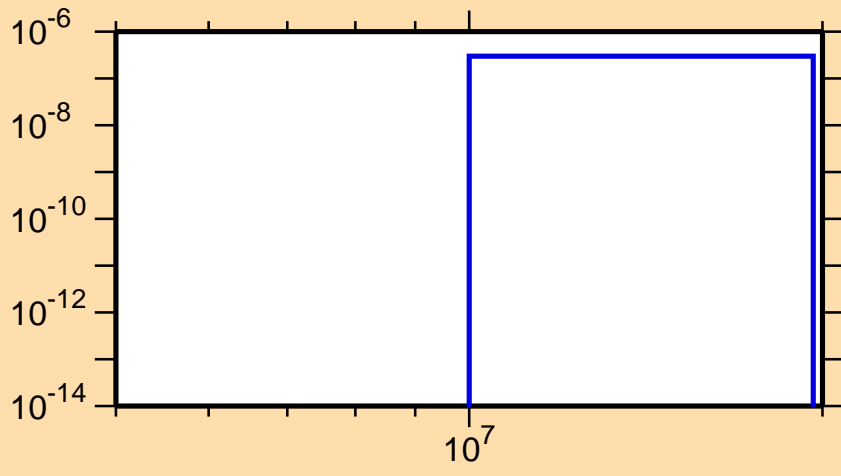
\sigma vs. E for ^{177}\text{Ir}(n,\text{nd})
