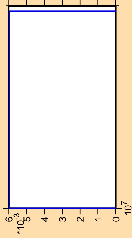
\Delta\sigma/\sigma vs. E for ^{177}\text{Ir}(n,3n\alpha)
