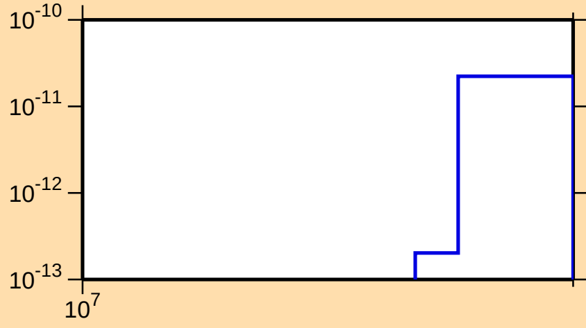
\sigma vs. E for ^{186}\text{Ir}(\text{mt } 34)
