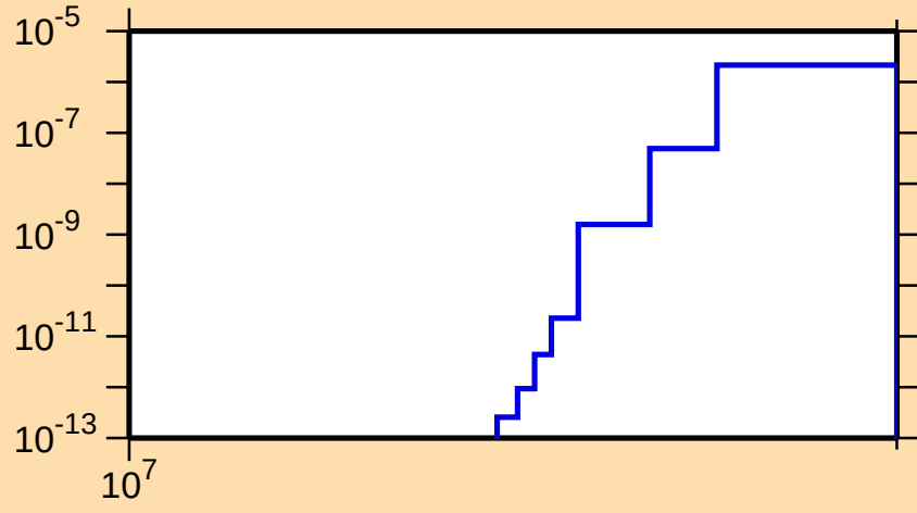
\sigma vs. E for ^{186}\text{Ir}(n,nt)
