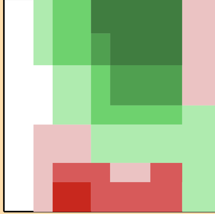
\Delta\sigma/\sigma vs. E for ^{186}\text{Ir}(n,2n)
