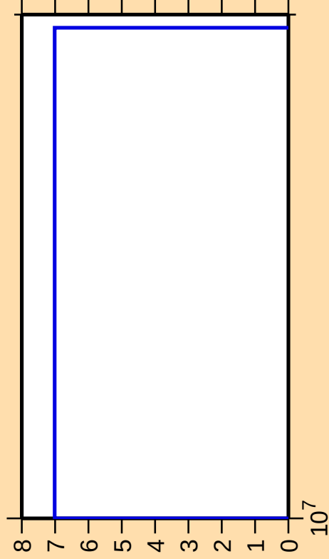
\Delta\sigma/\sigma vs. E for ^{186}\text{Ir}(\text{mt117})
