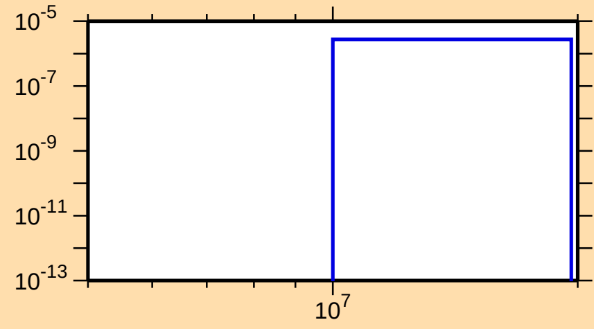
\sigma vs. E for ^{186}\text{Ir}(n,\text{nd})
