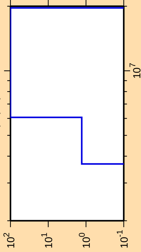
\Delta\sigma/\sigma vs. E for ^{186}\text{Ir}(n,p\alpha)
