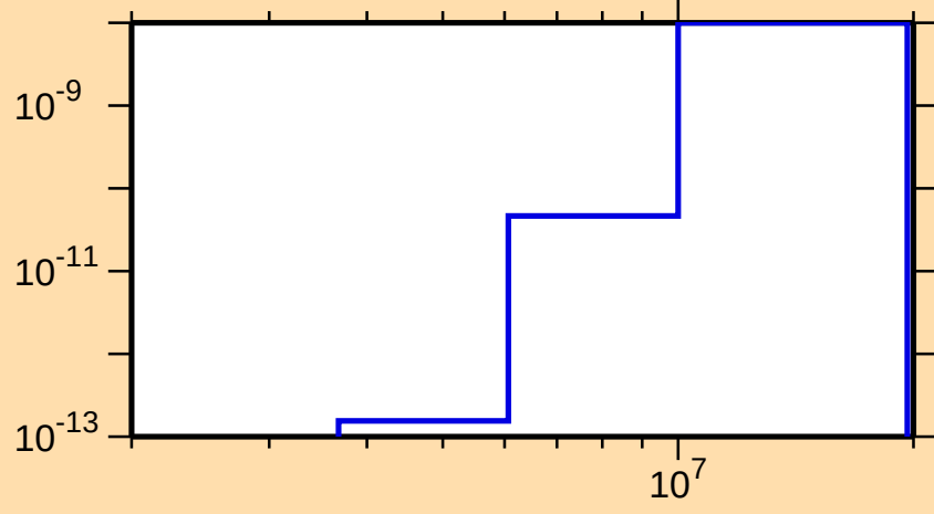
\sigma vs. E for ^{186}\text{Ir}(n,p\alpha)
