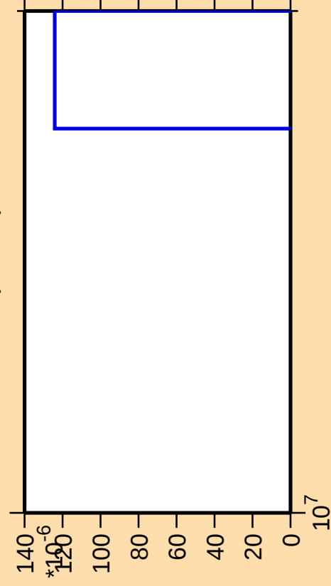
\Delta\sigma/\sigma vs. E for ^{187}\text{Ir}(\text{mt } 42)
