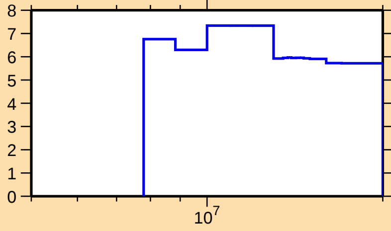
\Delta\sigma/\sigma vs. E for ^{187}\text{Ir}(n,\text{tot.})
