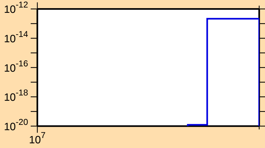
\sigma vs. E for ^{187}\text{Ir}(n,3n\alpha)
