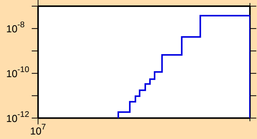
\sigma vs. E for ^{187}\text{Ir}(n,\text{He3})
