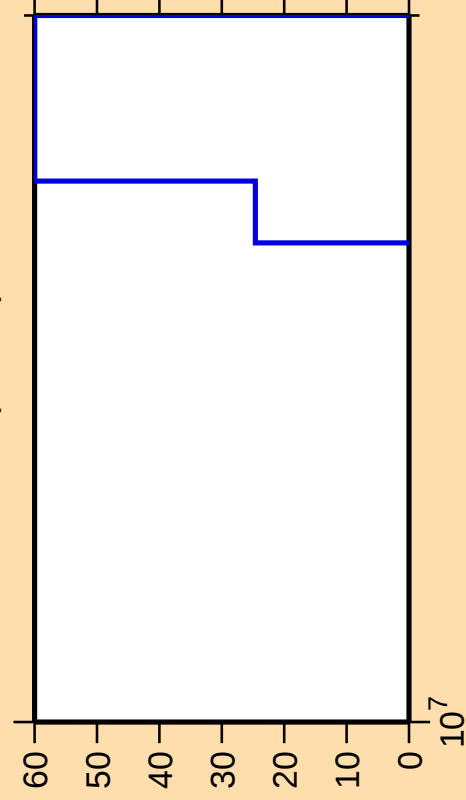
\Delta\sigma/\sigma vs. E for ^{187}\text{Ir}(\text{mt } 45)
