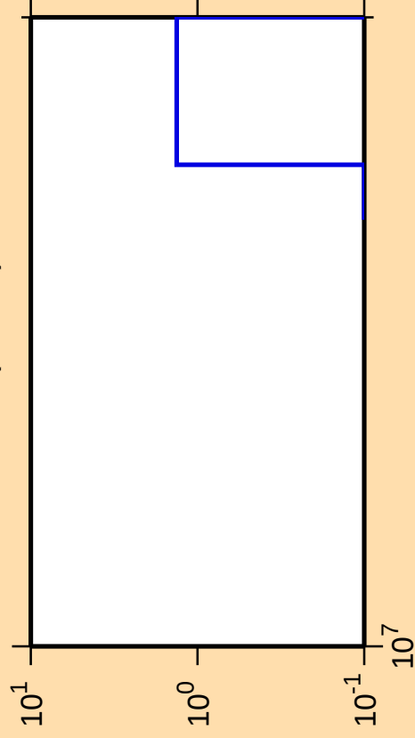
\Delta\sigma/\sigma vs. E for ^{187}\text{Ir}(n,3n\alpha)
