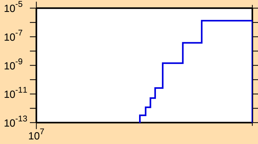
\sigma vs. E for ^{187}\text{Ir}(n,nt)
