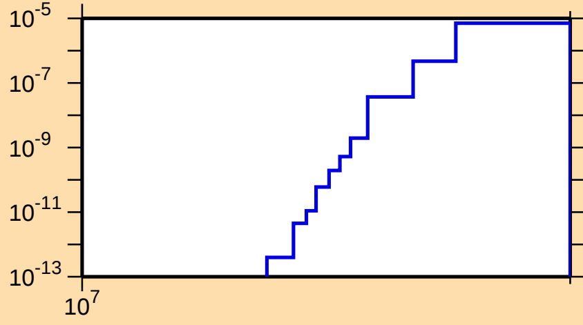
\sigma vs. E for ^{187}\text{Ir}(n,\text{nd})
