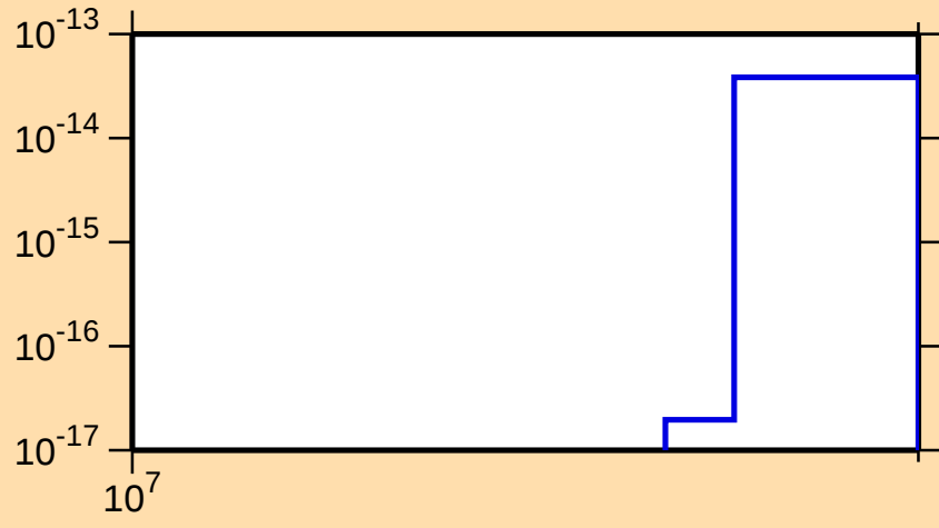
\sigma vs. E for ^{187}\text{Ir}(\text{mt } 34)
