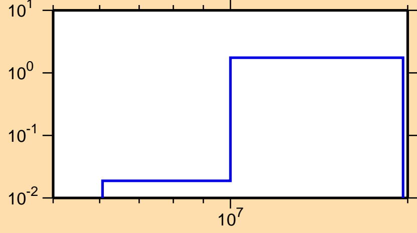
\sigma vs. E for ^{187}\text{Ir}(n,2n)
