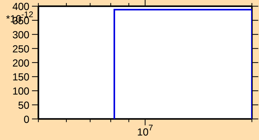
\sigma vs. E for ^{187}\text{Ir}(n,p\alpha)
