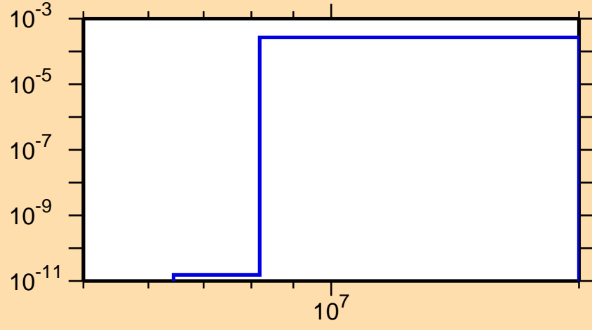
\sigma vs. E for ^{191}\text{Ir}(n,np)
