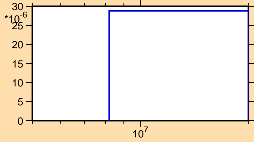
\sigma vs. E for ^{191}\text{Ir}(n,t)
