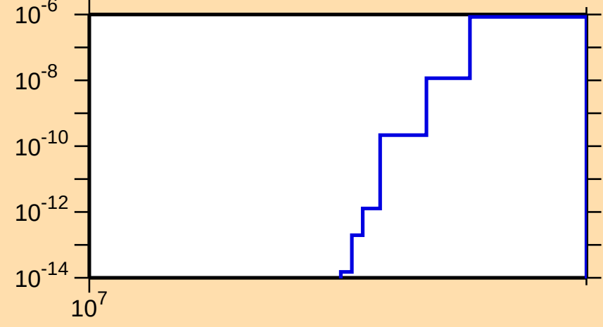
\sigma vs. E for ^{192}\text{Ir}(n,\text{nt})
