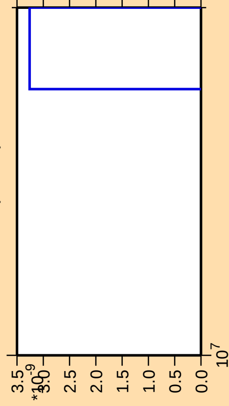
\Delta\sigma/\sigma vs. E for ^{192}\text{Ir}(\text{mt } 42)
