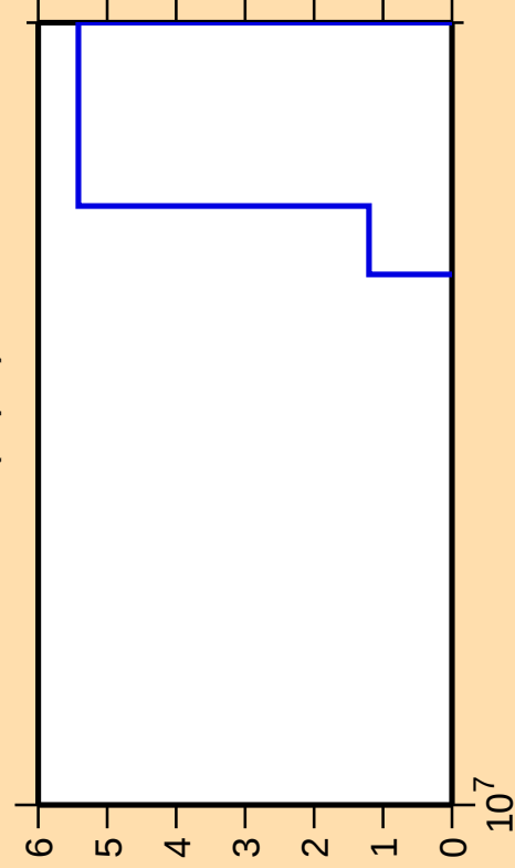
\Delta\sigma/\sigma vs. E for ^{192}\text{Ir}(n,p\alpha)
