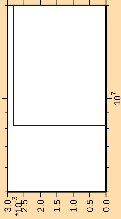
\Delta\sigma/\sigma vs. E for ^{192}\text{Ir}(n,3n\alpha)
