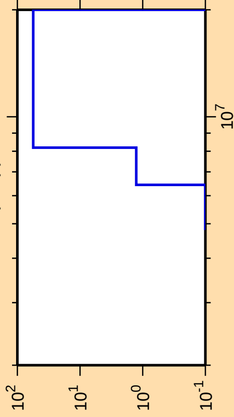
\Delta\sigma/\sigma vs. E for ^{192}\text{Ir}(n,np)
