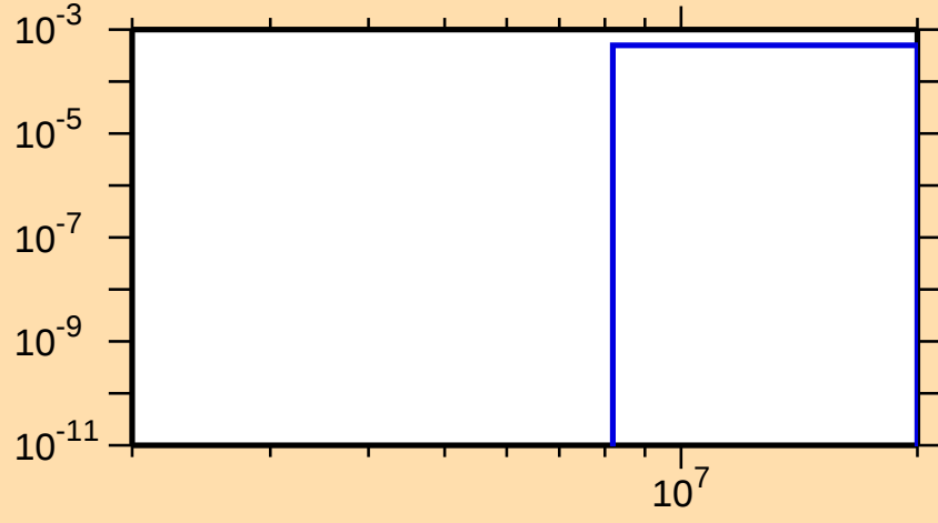
\sigma vs. E for ^{192}\text{Ir}(n,np)
