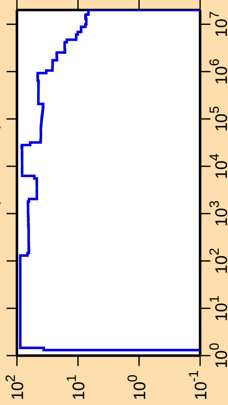
\Delta\sigma/\sigma vs. E for ^{193}\text{Ir}(n,\text{nonel.})
