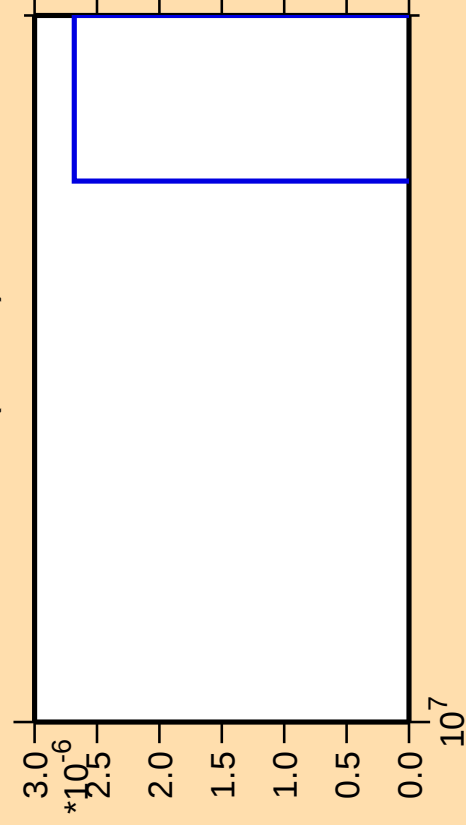
\Delta\sigma/\sigma vs. E for ^{193}\text{Ir}(\text{mt } 42)
