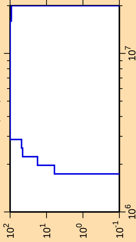
\Delta\sigma/\sigma vs. E for ^{193}\text{Ir}(n,\alpha)
