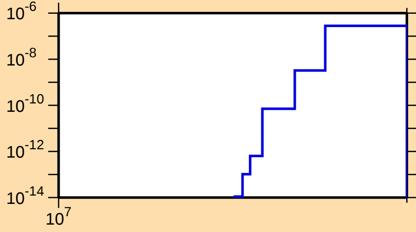
\sigma vs. E for ^{193}\text{Ir}(n,nt)
