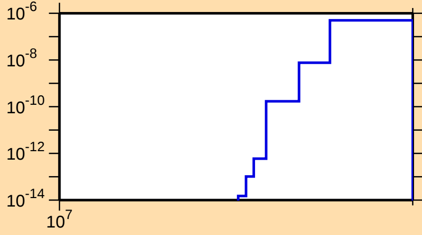
\sigma vs. E for ^{193}\text{Ir}(n,\text{nd})
