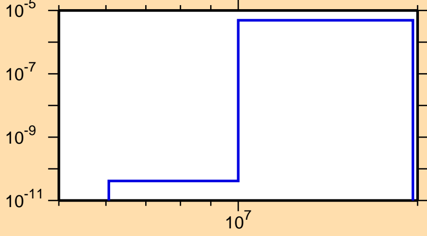
\sigma vs. E for ^{193}\text{Ir}(n,\alpha)
