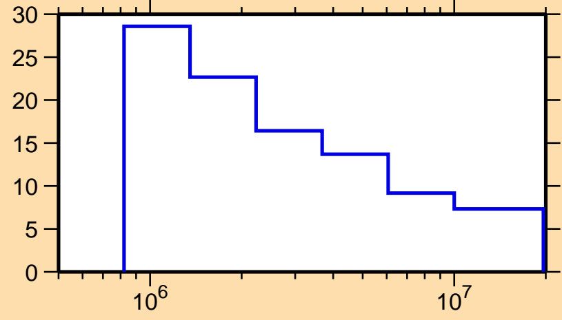
\Delta\sigma/\sigma vs. E for ^{193}\text{Ir}(n,n\text{onel.})
