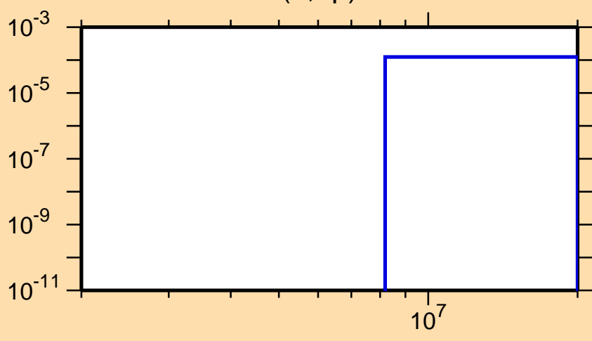
\sigma vs. E for ^{193}\text{Ir}(n,np)
