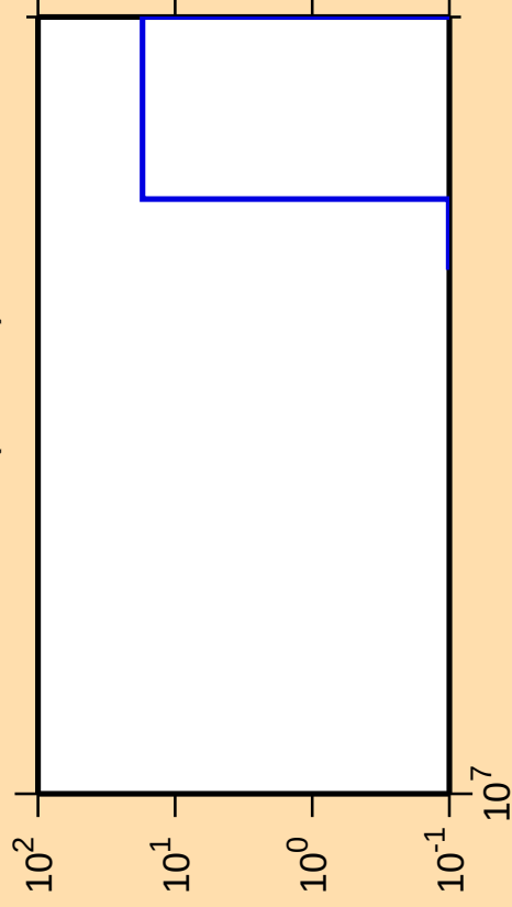
\Delta\sigma/\sigma vs. E for ^{194}\text{Ir}(n,\text{He}3)
