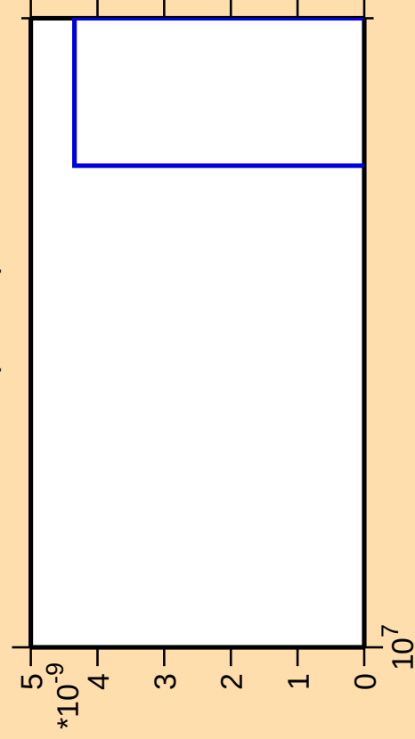
\Delta\sigma/\sigma vs. E for ^{194}\text{Ir}(\text{mt } 42)
