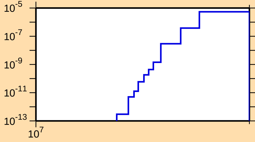
\sigma vs. E for ^{194}\text{Ir}(n,\text{nd})
