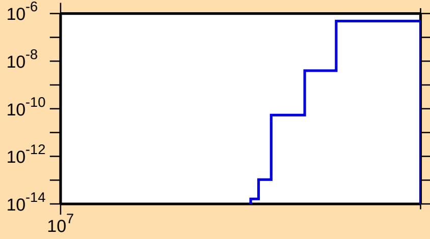
\sigma vs. E for ^{194}\text{Ir}(n,nt)
