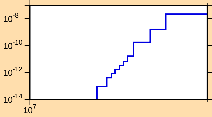
\sigma vs. E for ^{194}\text{Ir}(n,2n\alpha)
