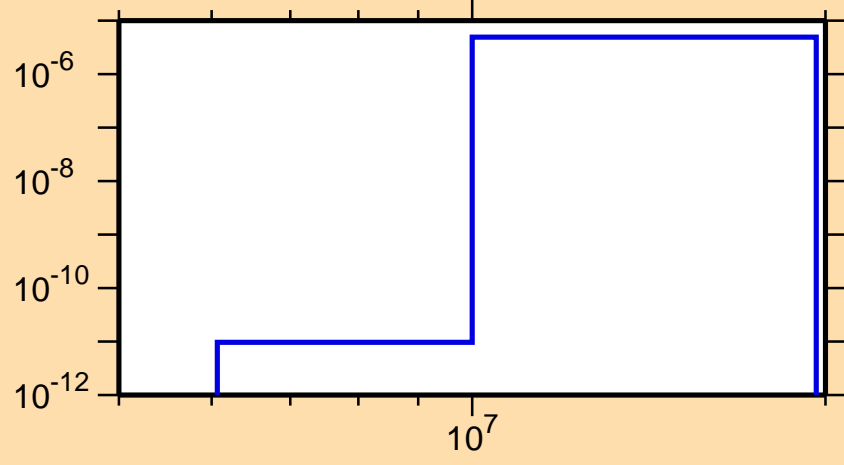
\sigma vs. E for ^{194}\text{Ir}(n,\alpha)
