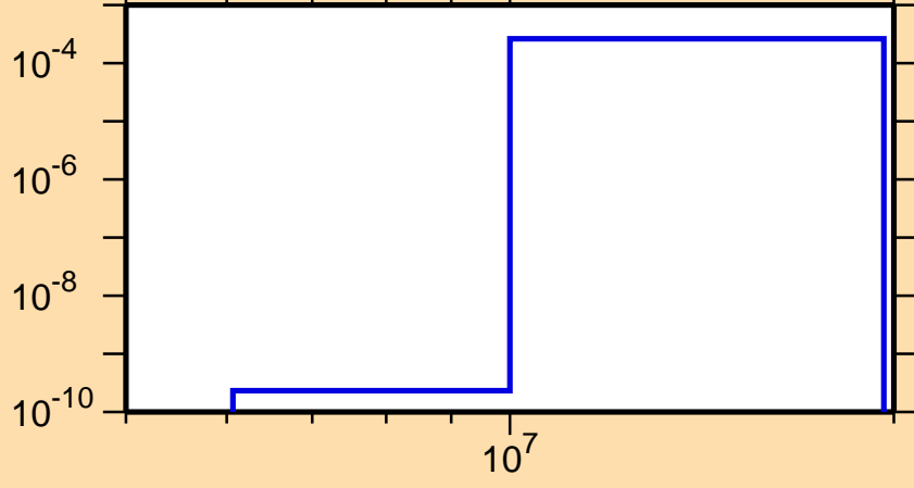
\sigma vs. E for ^{194}\text{Ir}(n,d)
