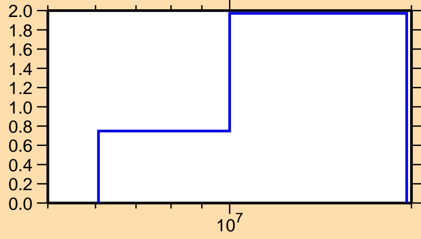
\sigma vs. E for ^{194}\text{Ir}(n,2n)
