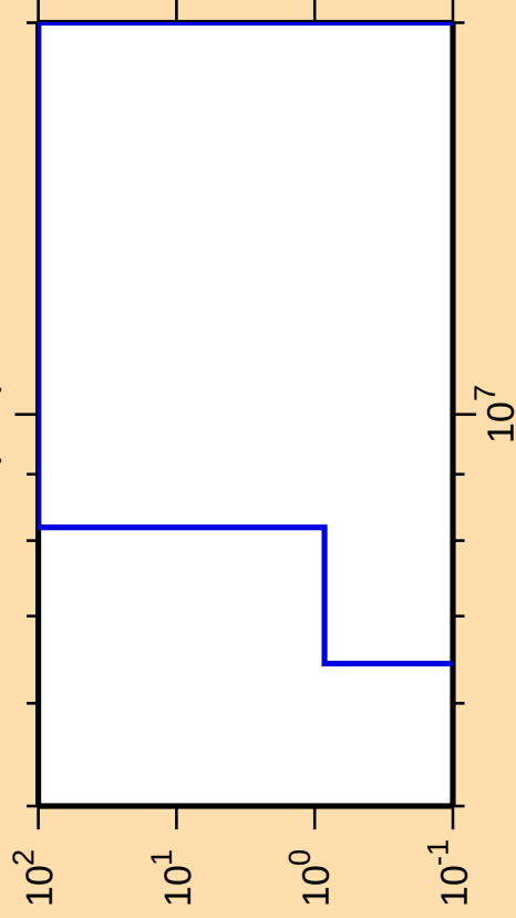
\Delta\sigma/\sigma vs. E for ^{194}\text{Ir}(n,d)
