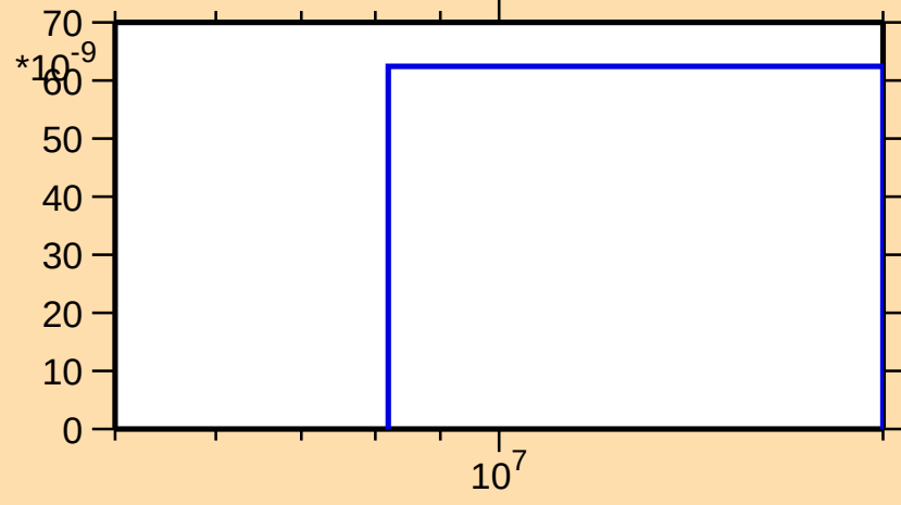
\sigma vs. E for ^{194}\text{Ir}(n,\text{nd})
