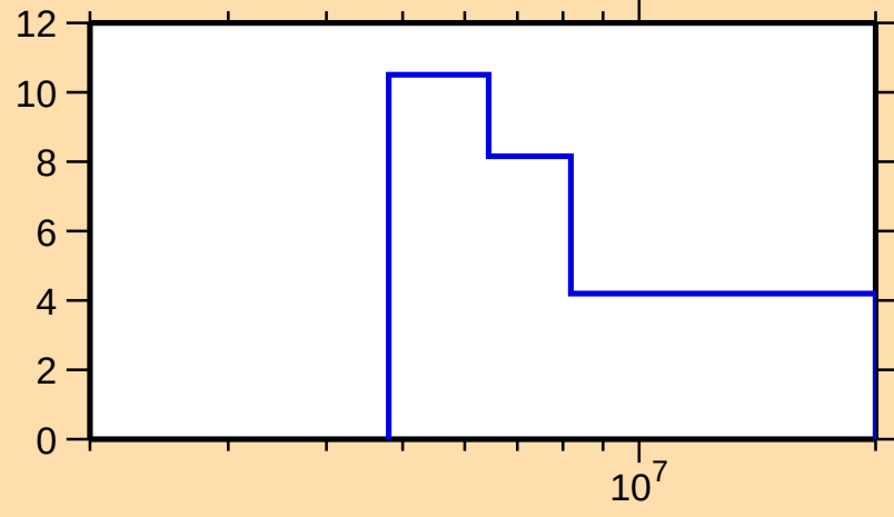
\Delta\sigma/\sigma vs. E for ^{194}\text{Ir}(n,\text{tot.})
