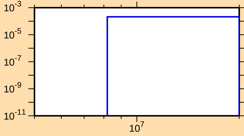
\sigma vs. E for ^{194}\text{Ir}(n,d)
