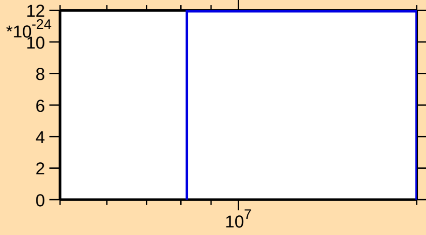
\sigma vs. E for ^{194}\text{Ir}(\text{mt } 42)
