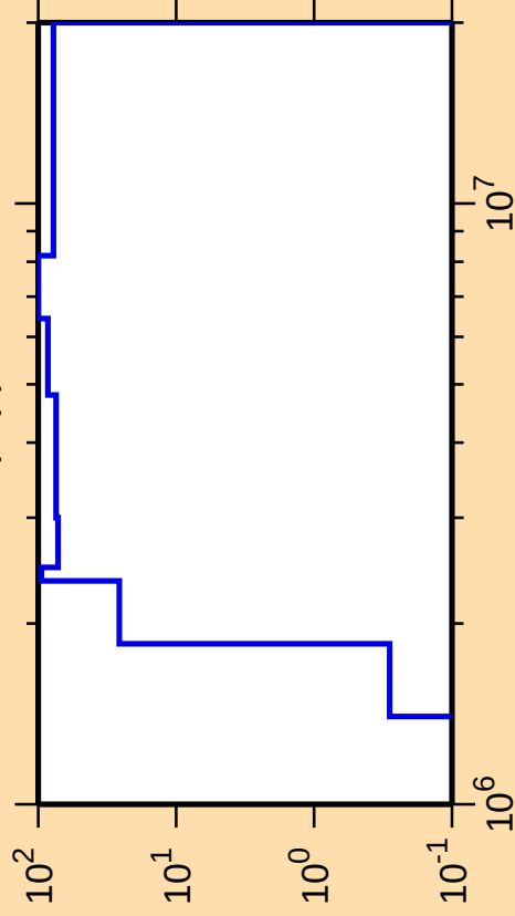
\Delta\sigma/\sigma vs. E for ^{194}\text{Ir}(n,p)
