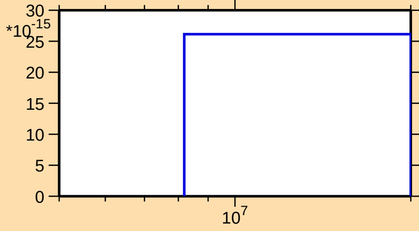
\sigma vs. E for ^{194}\text{Ir}(n,\text{He}3)
