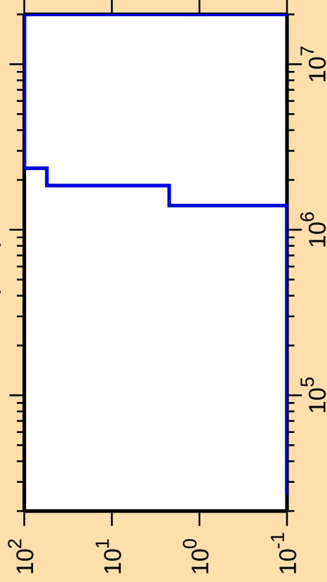
\Delta\sigma/\sigma vs. E for ^{194}\text{Ir}(n,\alpha)
