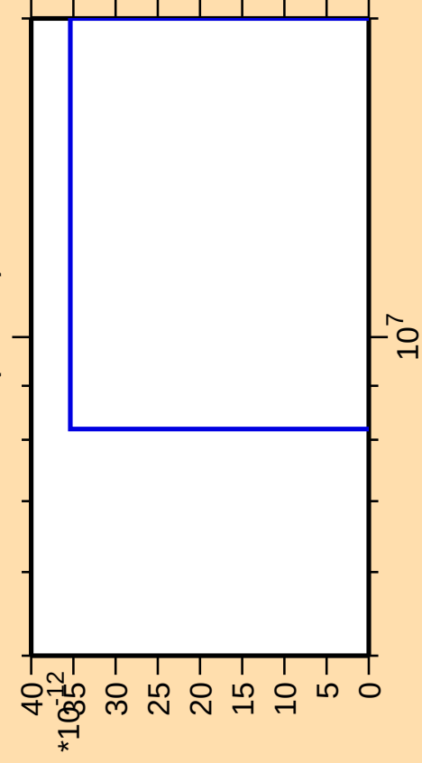
\Delta\sigma/\sigma vs. E for ^{194}\text{Ir}(\text{mt } 42)
