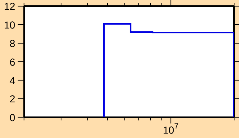
\Delta\sigma/\sigma vs. E for ^{194}\text{Ir}(n,\text{nonel.})
