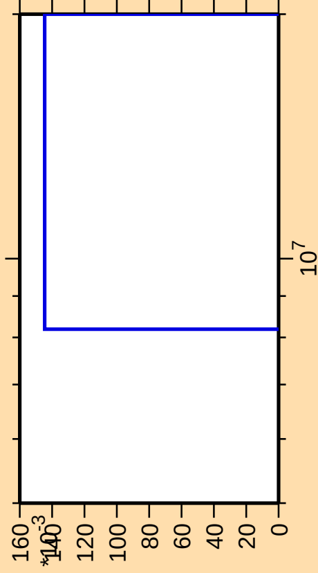
\Delta\sigma/\sigma vs. E for ^{194}\text{Ir}(n,\text{He}3)
