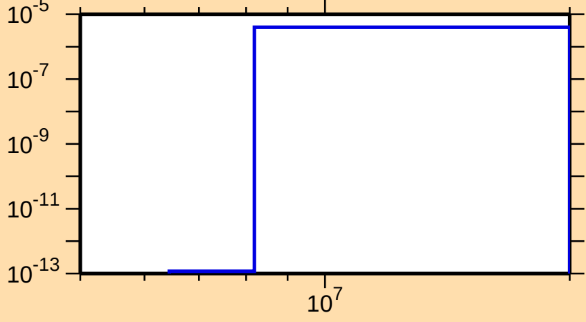
\sigma vs. E for ^{194}\text{Ir}(n,n\alpha)
