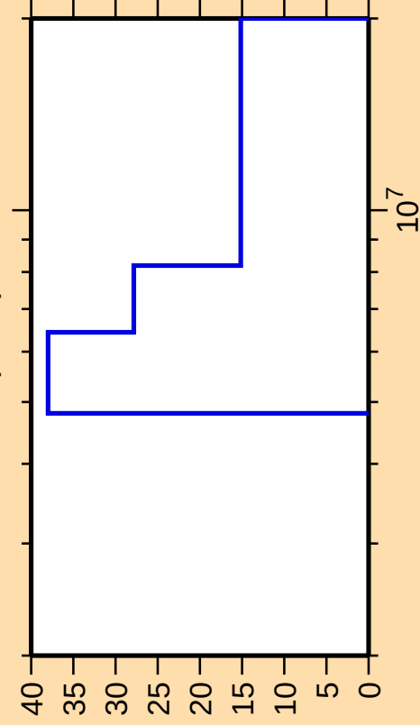
\Delta\sigma/\sigma vs. E for ^{194}\text{Ir}(n,2n)
