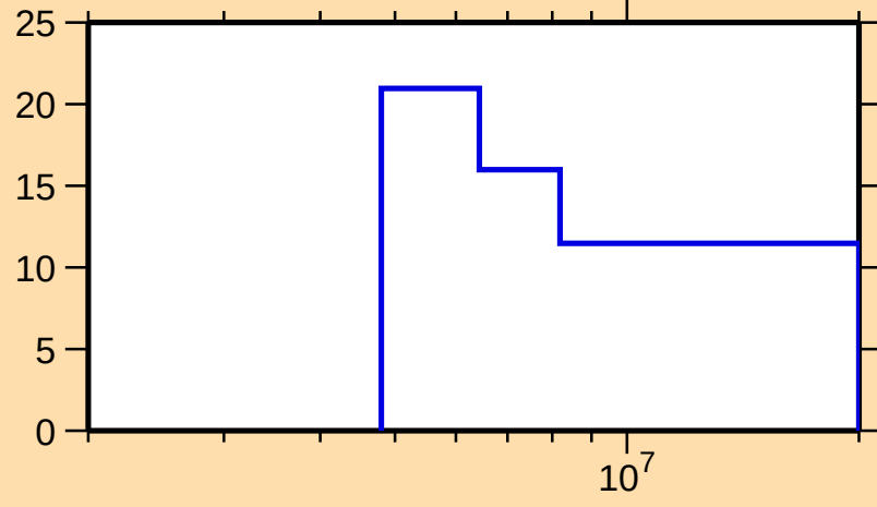
\Delta\sigma/\sigma vs. E for ^{194}\text{Ir}(n,\text{el.})
