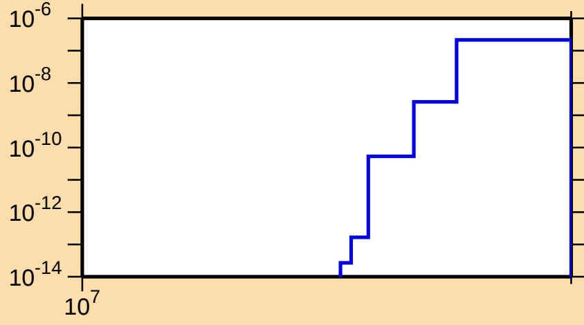
\sigma vs. E for ^{195}\text{Ir}(n,\text{nd})
