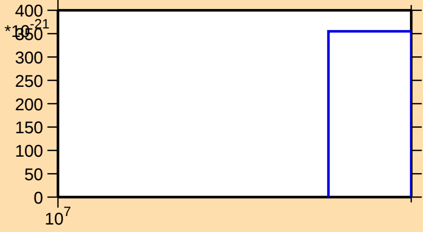
\sigma vs. E for ^{195}\text{Ir}(\text{mt } 42)
