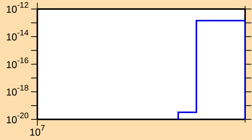
\sigma vs. E for ^{195}\text{Ir}(n,\text{He}3)
