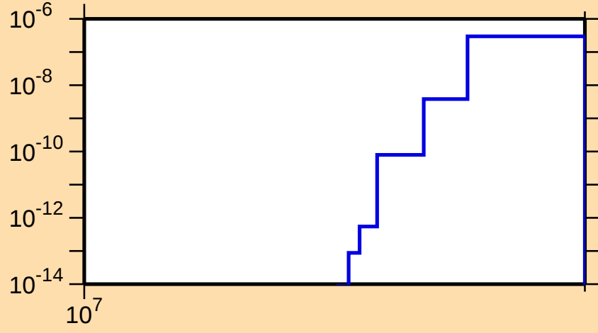
\sigma vs. E for ^{195}\text{Ir}(n,nt)
