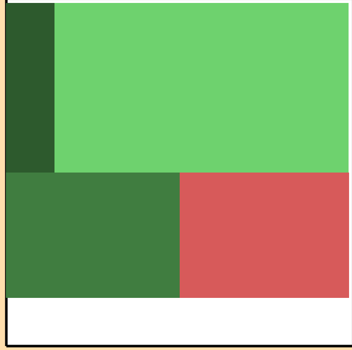
\Delta\sigma/\sigma vs. E for ^{195}\text{Ir}(n,\text{tot.})
