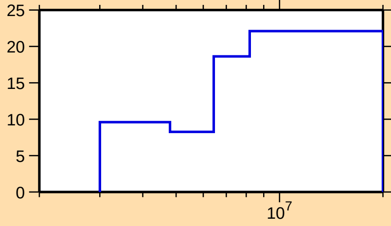
\Delta\sigma/\sigma vs. E for ^{195}\text{Ir}(n,n\text{cont.})
