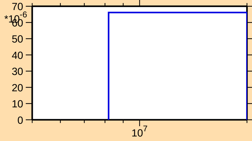
\sigma vs. E for ^{195}\text{Ir}(n,np)
