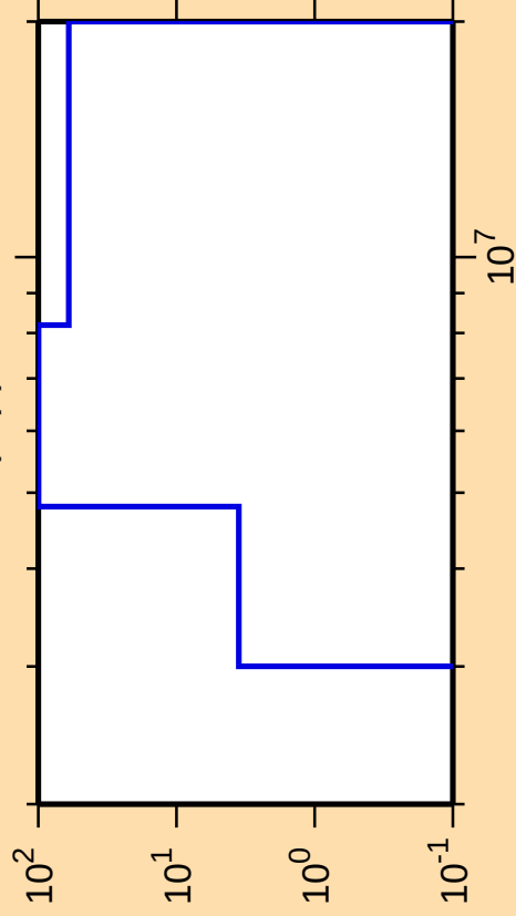
\Delta\sigma/\sigma vs. E for ^{195}\text{Ir}(n,p)
