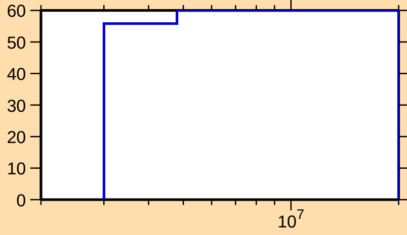
\Delta\sigma/\sigma vs. E for ^{195}\text{Ir}(n,n_1)
