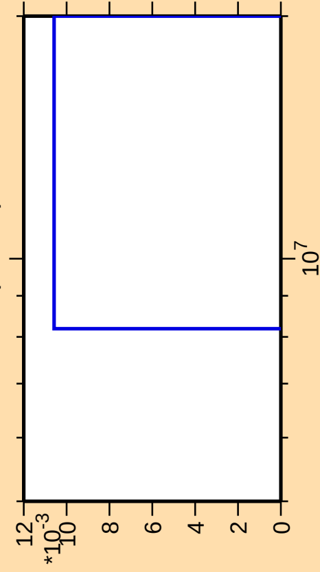
\Delta\sigma/\sigma vs. E for ^{195}\text{Ir}(n,\text{He}3)
