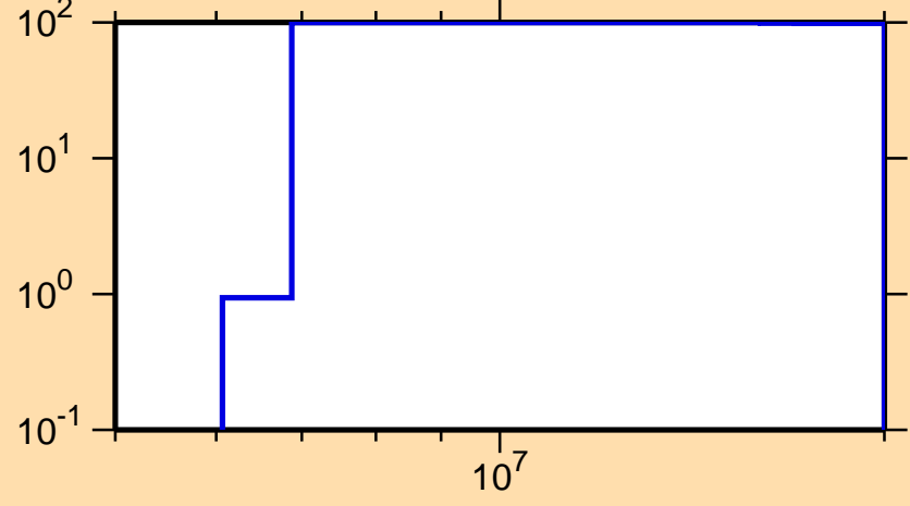
\Delta\sigma/\sigma vs. E for ^{201}\text{Ir}(n,p)
