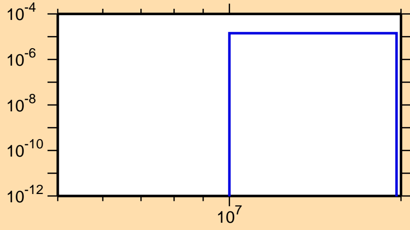
\sigma vs. E for ^{201}\text{Ir}(n,np)
