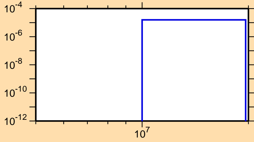
\sigma vs. E for ^{201}\text{Ir}(n,d)
