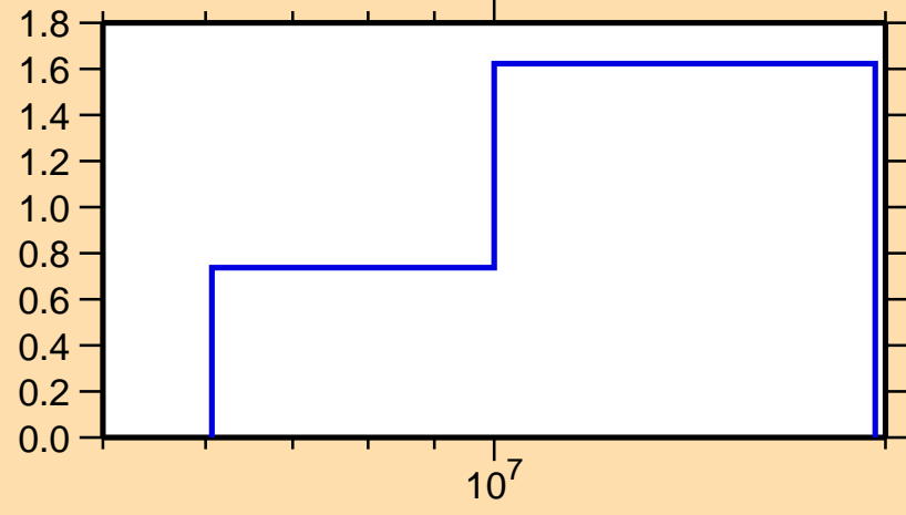
\sigma vs. E for ^{201}\text{Ir}(n,2n)
