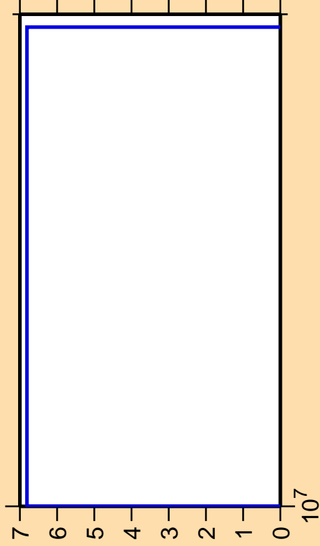
\Delta\sigma/\sigma vs. E for ^{201}\text{Ir}(n,2np)
