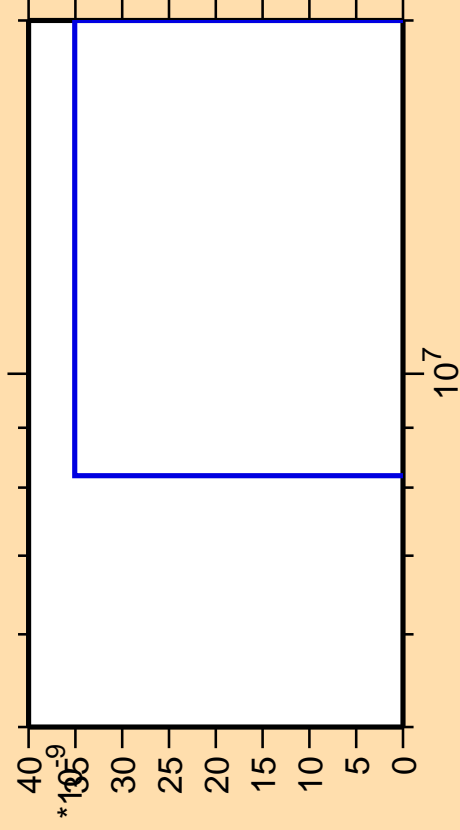
\Delta\sigma/\sigma vs. E for ^{201}\text{Ir}(\text{mt } 42)
