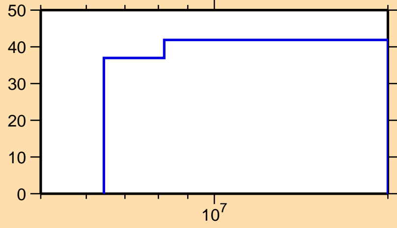
\Delta\sigma/\sigma vs. E for ^{201}\text{Ir}(n,ncont.)
