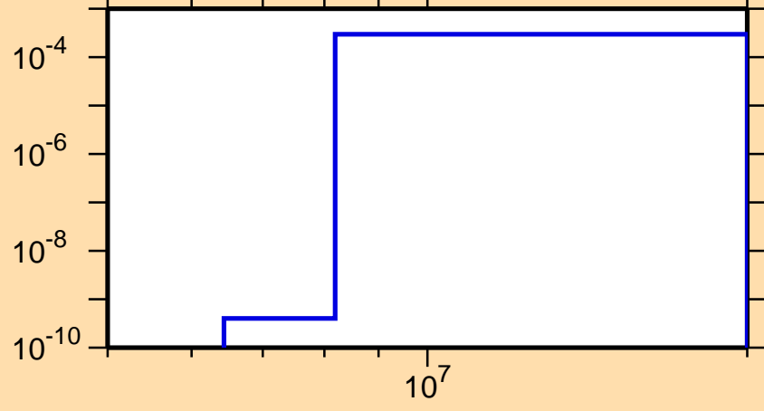
\sigma vs. E for ^{201}\text{Ir}(n,p)
