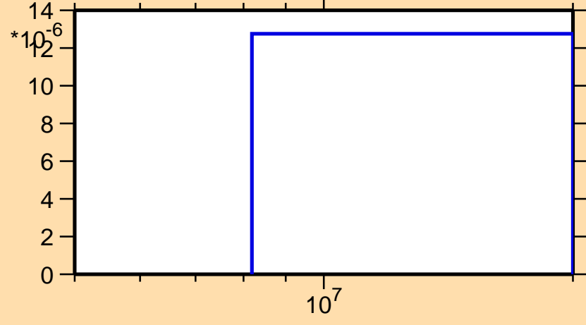
\sigma vs. E for ^{201}\text{Ir}(n,d)
