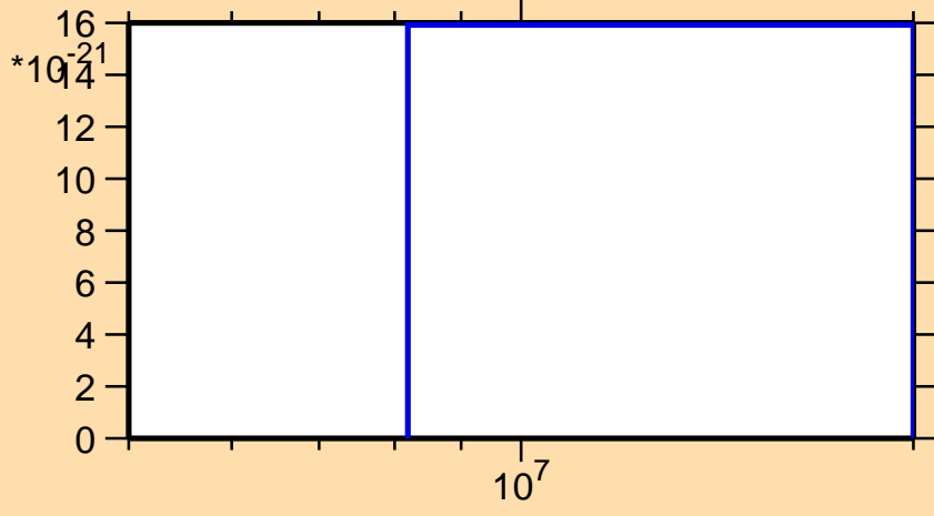
\sigma vs. E for ^{201}\text{Ir}(\text{mt } 42)
