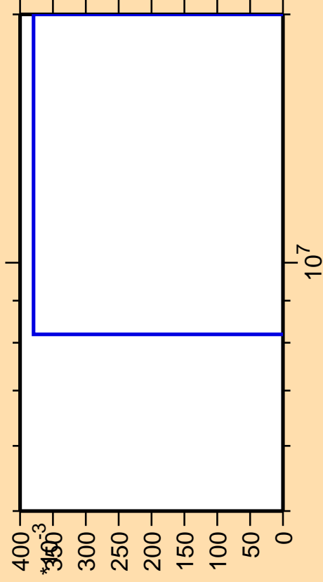
\Delta\sigma/\sigma vs. E for ^{201}\text{Ir}(n,2n\alpha)
