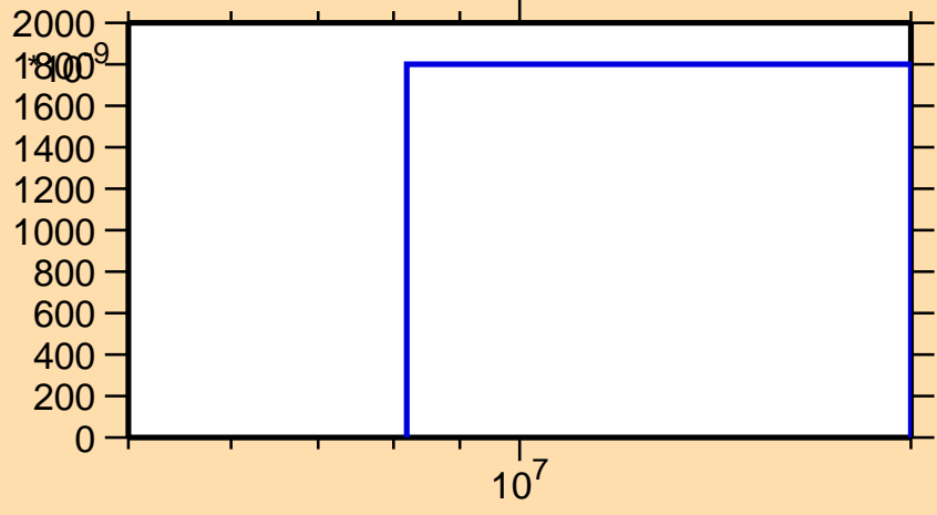
\sigma vs. E for ^{201}\text{Ir}(n,t)
