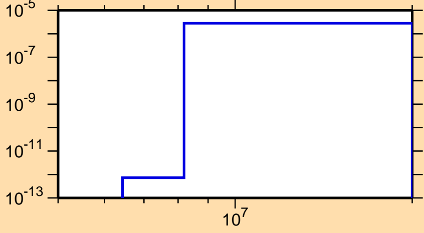
\sigma vs. E for ^{201}\text{Ir}(n,\alpha)
