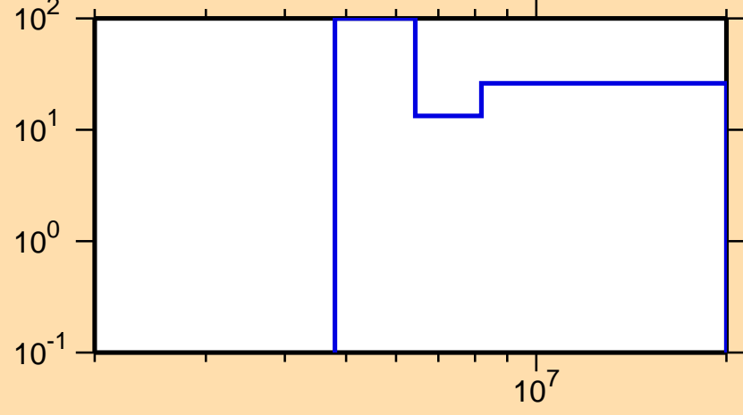
\Delta\sigma/\sigma vs. E for ^{201}\text{Ir}(n,2n)
