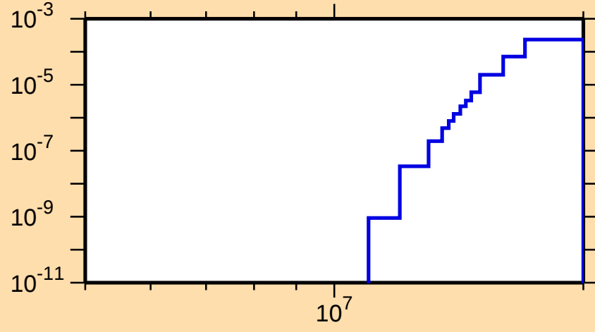
\sigma vs. E for ^{203}\text{Ir}(n,d)
