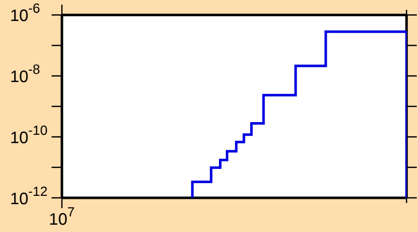
\sigma vs. E for ^{203}\text{Ir}(n,n\alpha)
