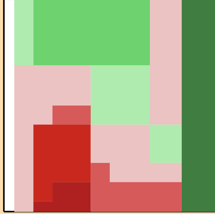
\Delta\sigma/\sigma vs. E for ^{203}\text{Ir}(n,2n)
