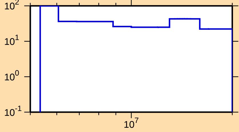
\Delta\sigma/\sigma vs. E for ^{203}\text{Ir}(n,2n)
