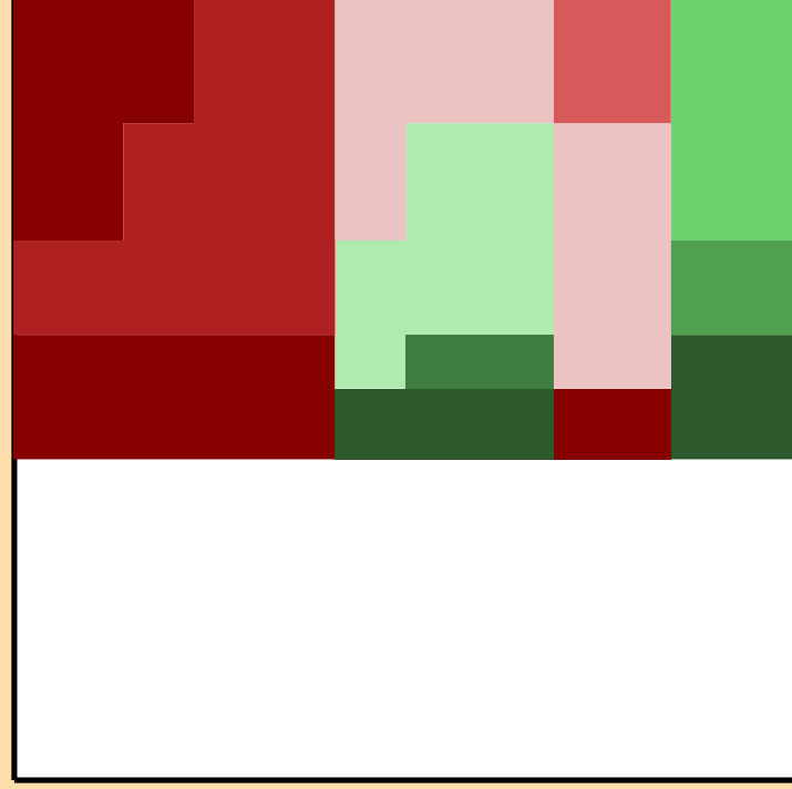
\Delta\sigma/\sigma vs. E for ^{203}\text{Ir}(n,\text{nonel.})
