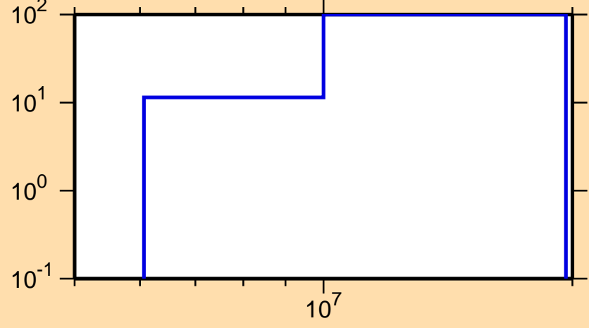
\Delta\sigma/\sigma vs. E for ^{203}\text{Ir}(n,p)
