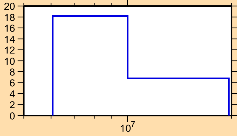
\Delta\sigma/\sigma vs. E for ^{203}\text{Ir}(n,el.)
