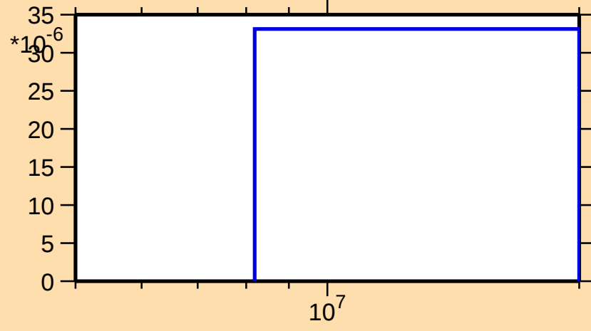
\sigma vs. E for ^{203}\text{Ir}(n,p)
