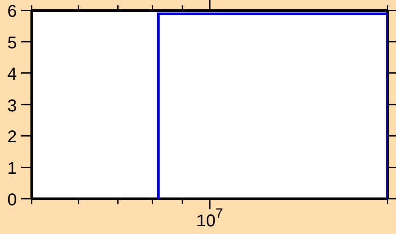
\Delta\sigma/\sigma vs. E for ^{203}\text{Ir}(n,\text{tot.})
