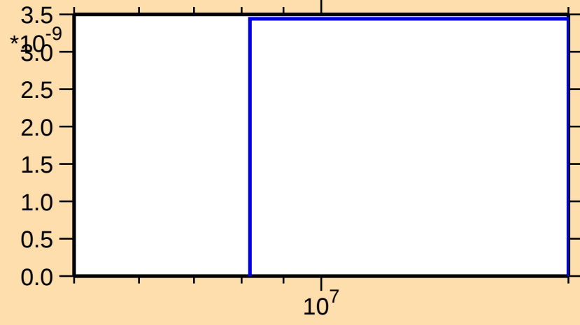
\sigma vs. E for ^{203}\text{Ir}(n,n\alpha)
