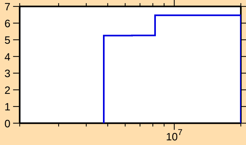
\Delta\sigma/\sigma vs. E for ^{203}\text{Ir}(n,\text{nonel.})
