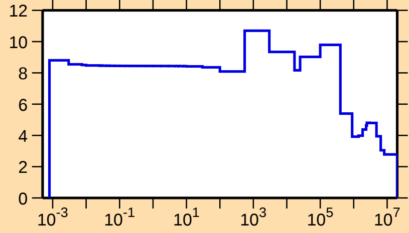
\sigma vs. E for ^{203}\text{Ir}(n,\text{el.})
