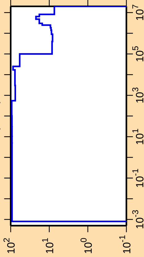
\Delta\sigma/\sigma vs. E for ^{203}\text{Ir}(n,\text{el.})
