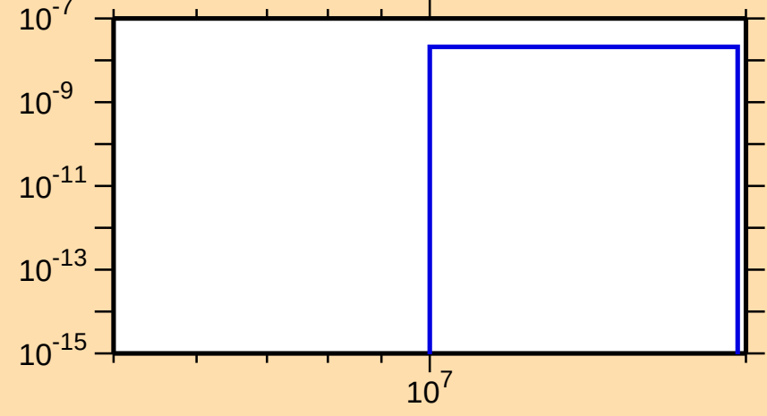
\sigma vs. E for ^{72}\text{Kr}(\text{mt117})
