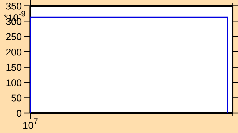
\sigma vs. E for ^{72}\text{Kr}(n,\text{pt})
