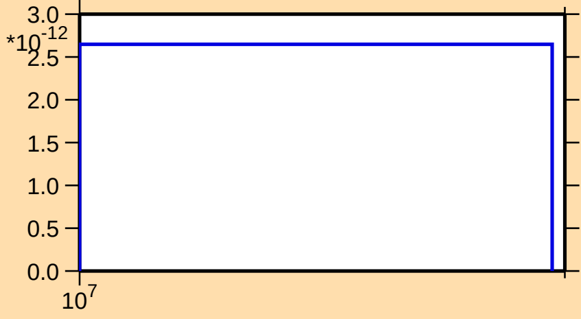
\sigma vs. E for ^{72}\text{Kr}(n,2np)
