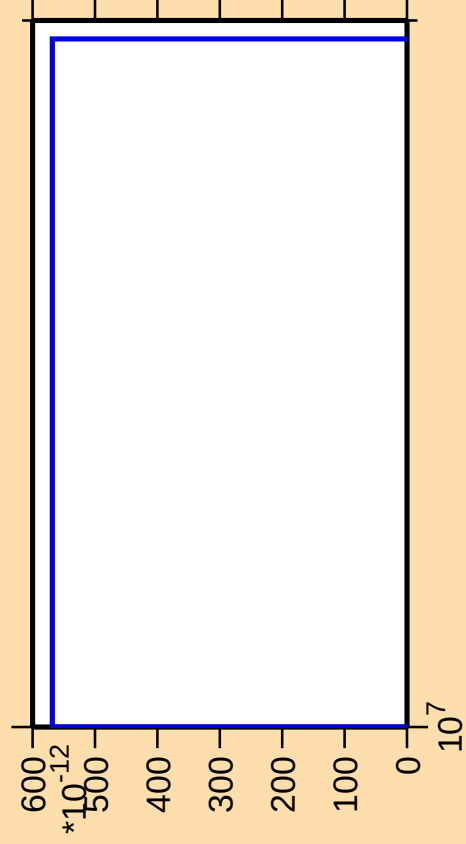
\Delta\sigma/\sigma vs. E for ^{72}\text{Kr}(n,2n\alpha)
