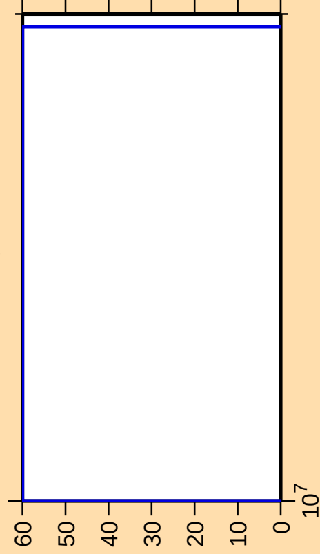
\Delta\sigma/\sigma vs. E for ^{72}\text{Kr}(n,\gamma)
