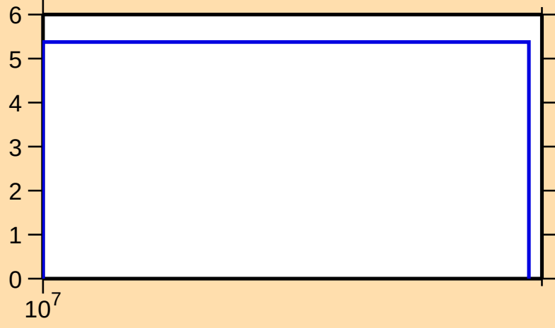
\Delta\sigma/\sigma vs. E for ^{72}\text{Kr}(n,\text{tot.})
