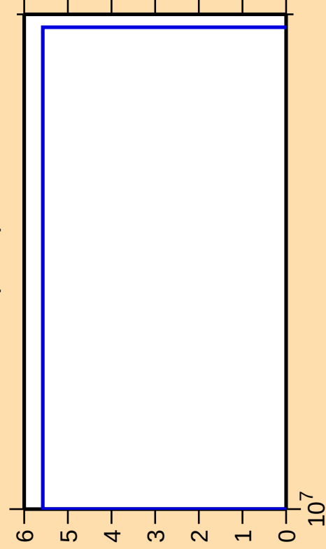
\Delta\sigma/\sigma vs. E for ^{72}\text{Kr}(n,\text{nd})
