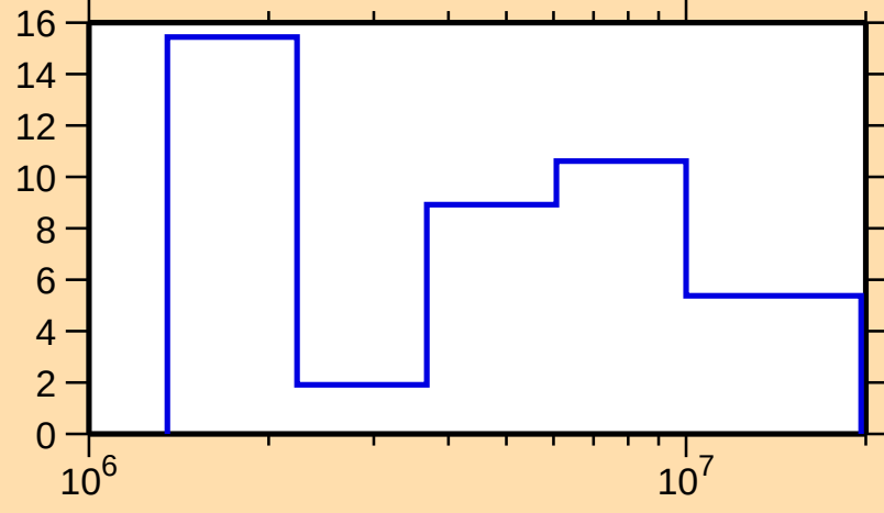
\Delta\sigma/\sigma vs. E for ^{72}\text{Kr}(n,\text{tot.})
