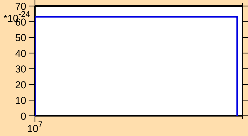
\sigma vs. E for ^{72}\text{Kr}(n,2n\alpha)
