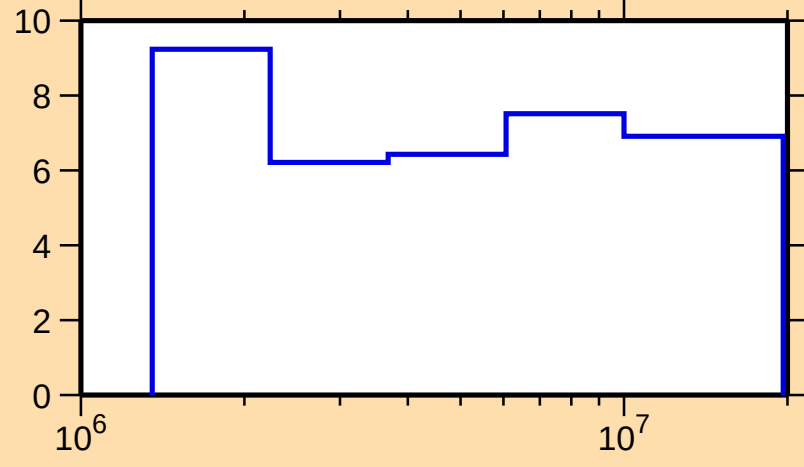
\Delta\sigma/\sigma vs. E for ^{72}\text{Kr}(n,\text{nonel.})
