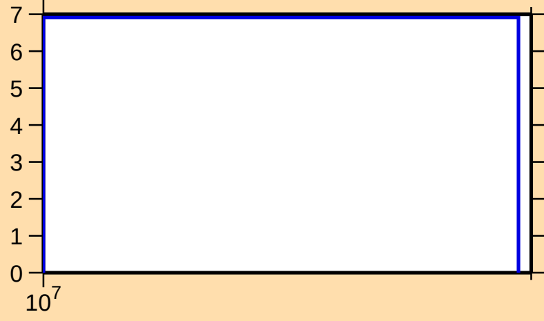
\Delta\sigma/\sigma vs. E for ^{72}\text{Kr}(n,\text{nonel.})
