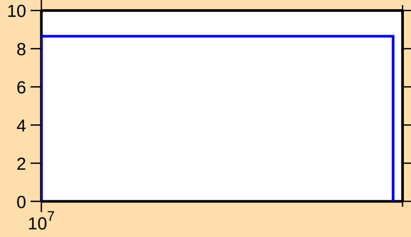
\Delta\sigma/\sigma vs. E for ^{72}\text{Kr}(n,\text{el.})
