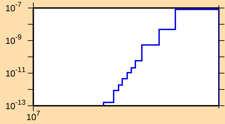
\sigma vs. E for ^{74}\text{Kr}(\text{mt117})
