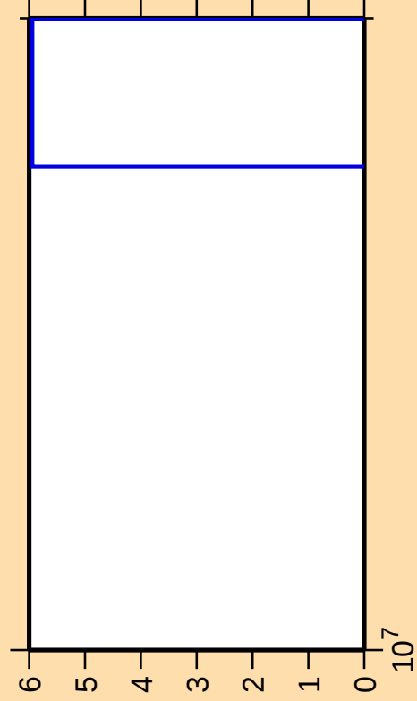
\Delta\sigma/\sigma vs. E for ^{74}\text{Kr}(n,2np)
