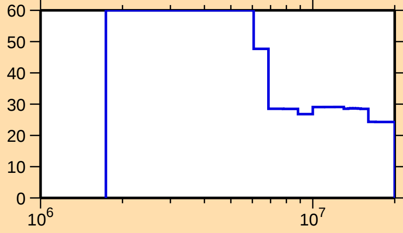
\Delta\sigma/\sigma vs. E for ^{74}\text{Kr}(n,n\text{cont.})
