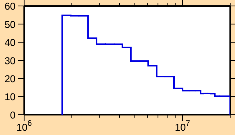
\Delta\sigma/\sigma vs. E for ^{74}\text{Kr}(n,\text{inel.})
