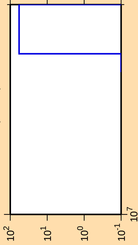
\Delta\sigma/\sigma vs. E for ^{74}\text{Kr}(\text{mt } 34)
