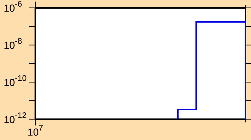
\sigma vs. E for ^{74}\text{Kr}(n,\text{pt})
