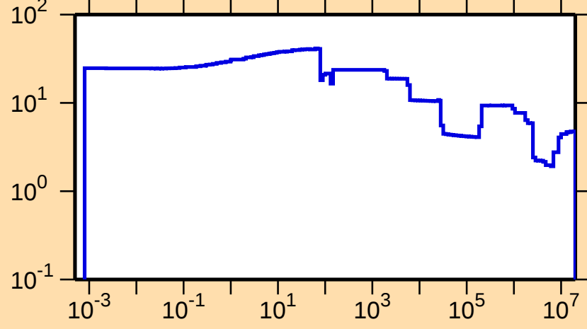
\Delta\sigma/\sigma vs. E for ^{74}\text{Kr}(\text{n,tot.})
