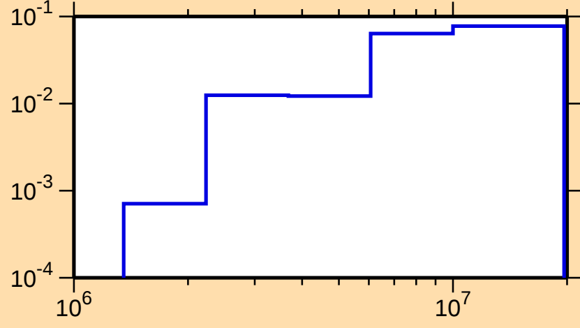
\sigma vs. E for ^{74}\text{Kr}(n,n\text{cont.})
