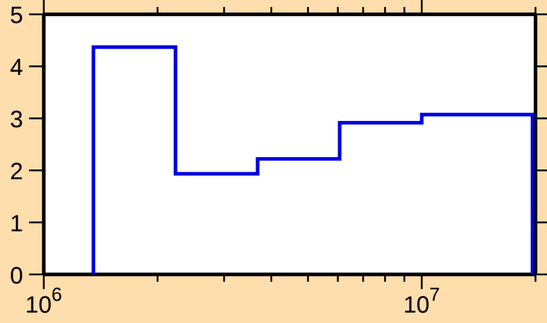
\Delta\sigma/\sigma vs. E for ^{74}\text{Kr}(n,\text{nonel.})
