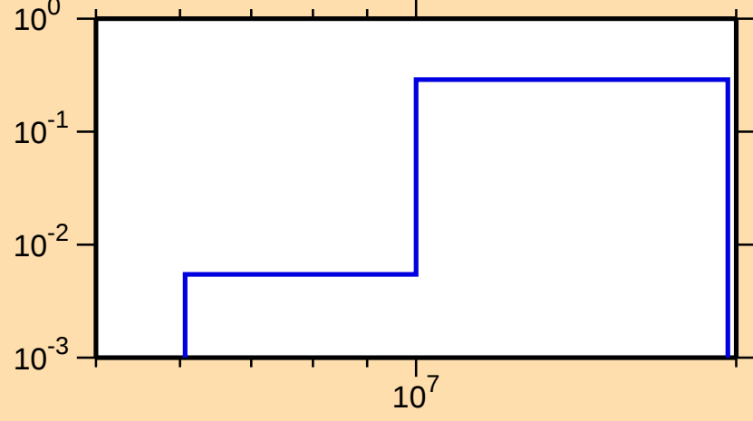
\sigma vs. E for ^{74}\text{Kr}(n,np)
