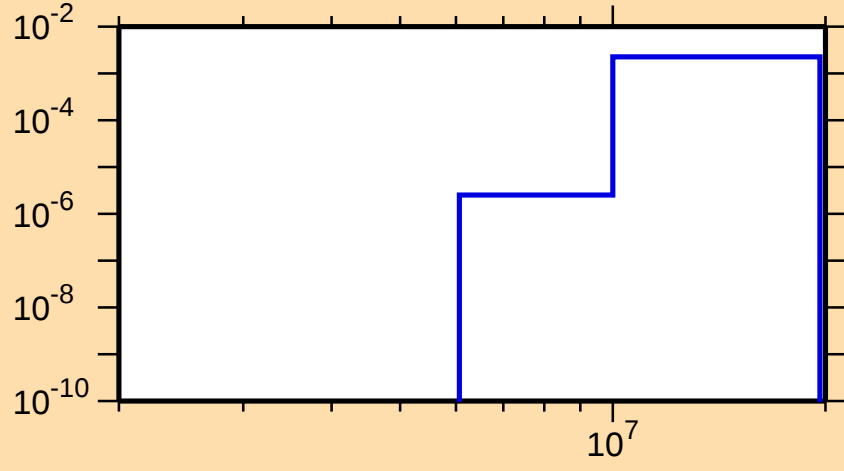
\sigma vs. E for ^{74}\text{Kr}(n,n\alpha)
