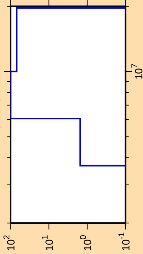
\Delta\sigma/\sigma vs. E for ^{74}\text{Kr}(n,n\alpha)
