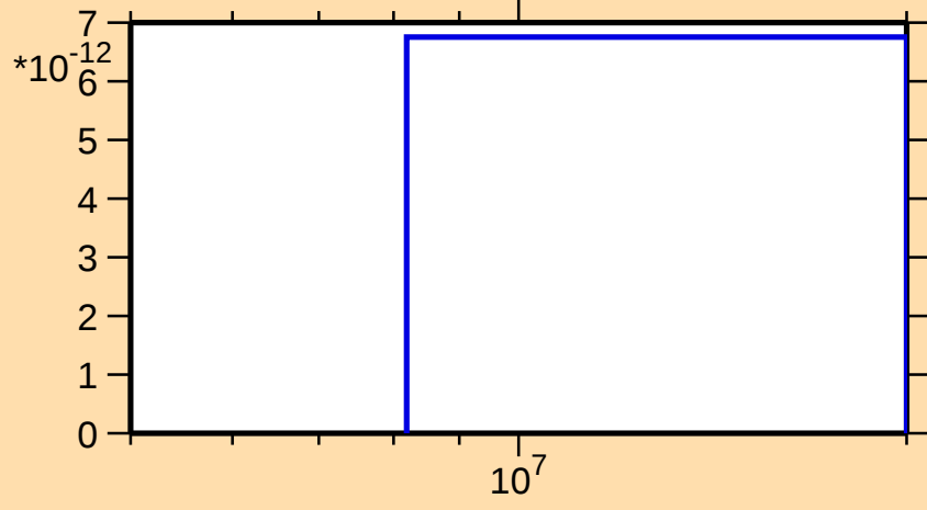
\sigma vs. E for ^{74}\text{Kr}(n,\text{nd})
