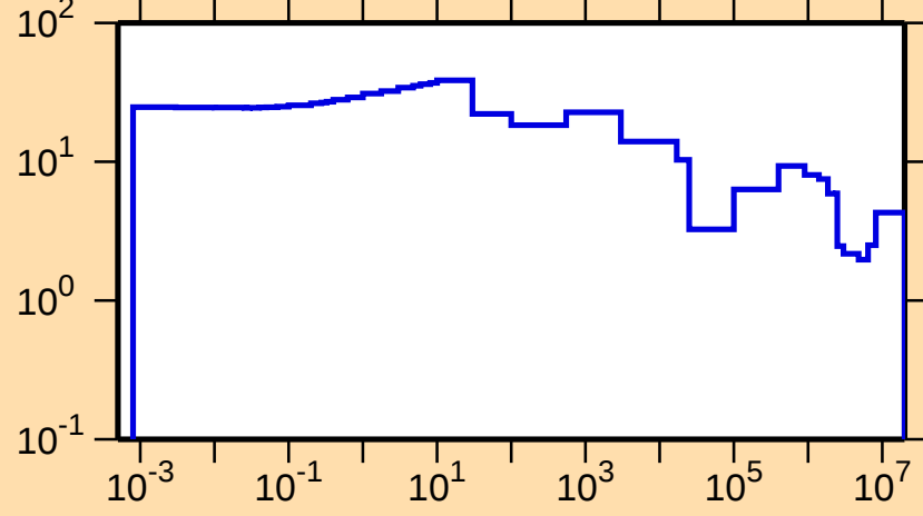
\Delta\sigma/\sigma vs. E for ^{74}\text{Kr}(\text{n,tot.})
