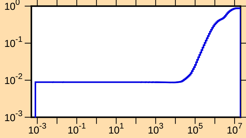
\mu vs. E for ^{76}\text{Kr}(\text{mt251})
