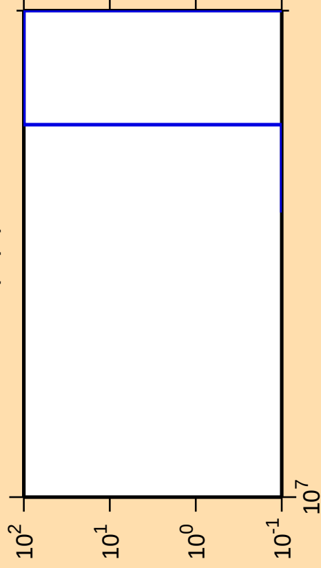
\Delta\sigma/\sigma vs. E for ^{76}\text{Kr}(n,\text{pt})
