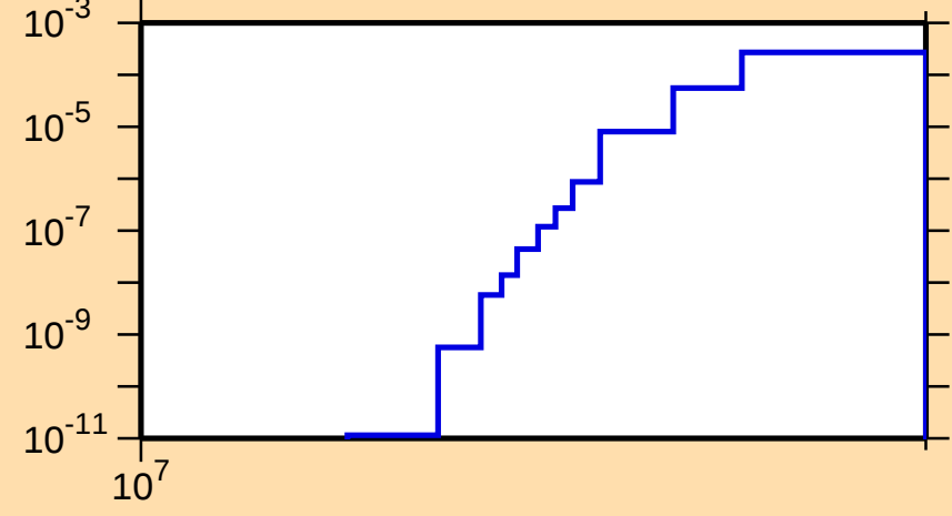
\sigma vs. E for ^{76}\text{Kr}(n,t)
