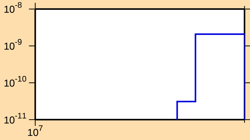
\sigma vs. E for ^{76}\text{Kr}(\text{mt117})
