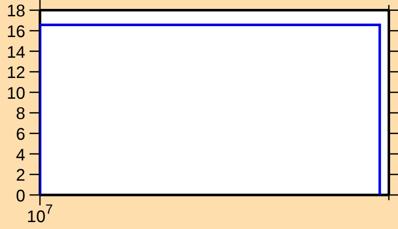
\Delta\sigma/\sigma vs. E for ^{76}\text{Kr}(n,\text{inel.})
