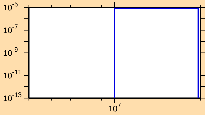
\sigma vs. E for ^{76}\text{Kr}(n,\text{pd})
