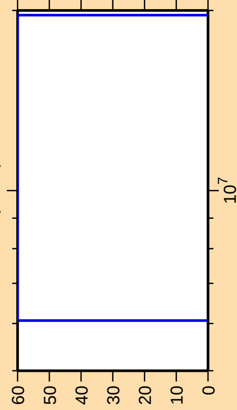
\Delta\sigma/\sigma vs. E for ^{76}\text{Kr}(n,n\alpha)
