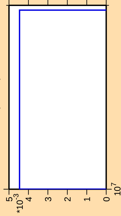
\Delta\sigma/\sigma vs. E for ^{76}\text{Kr}(\text{mt } 34)
