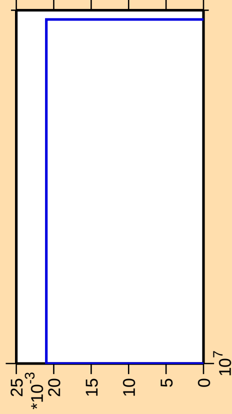
\Delta\sigma/\sigma vs. E for ^{76}\text{Kr}(n,2np)
