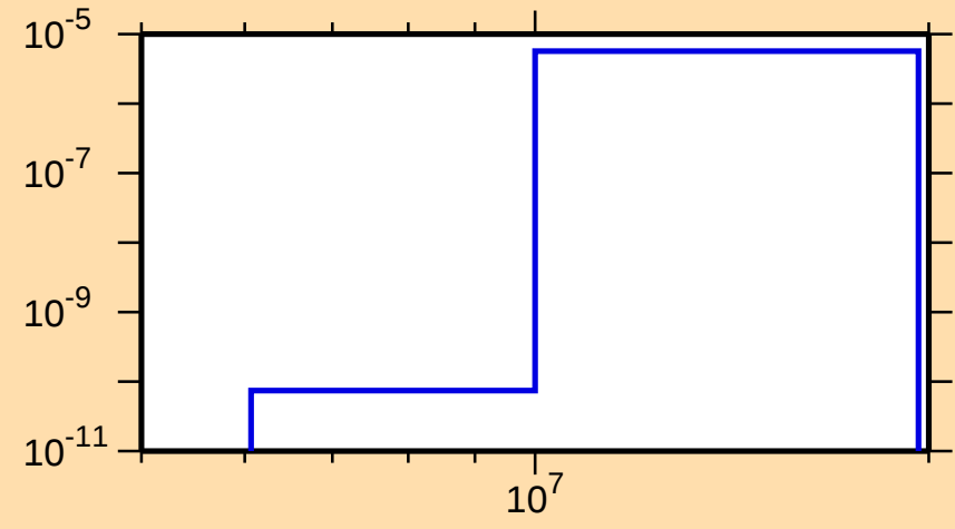
\sigma vs. E for ^{76}\text{Kr}(n,\text{He3})
