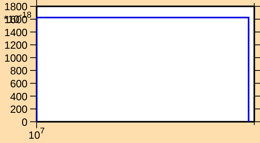
\sigma vs. E for ^{76}\text{Kr}(n,2np)
