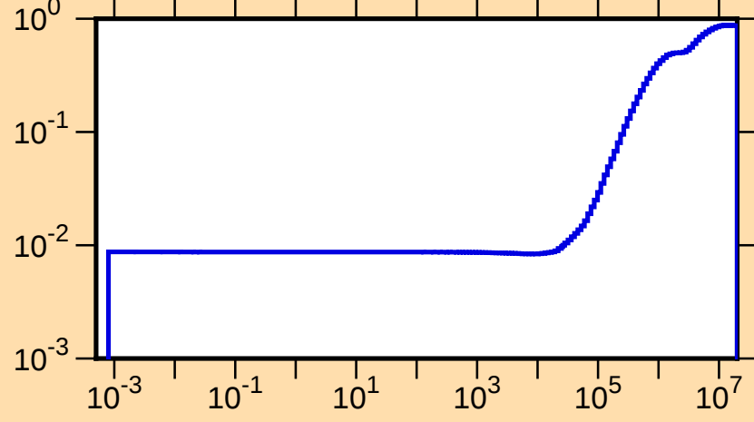
\mu vs. E for ^{77}\text{Kr}(\text{mt251})
