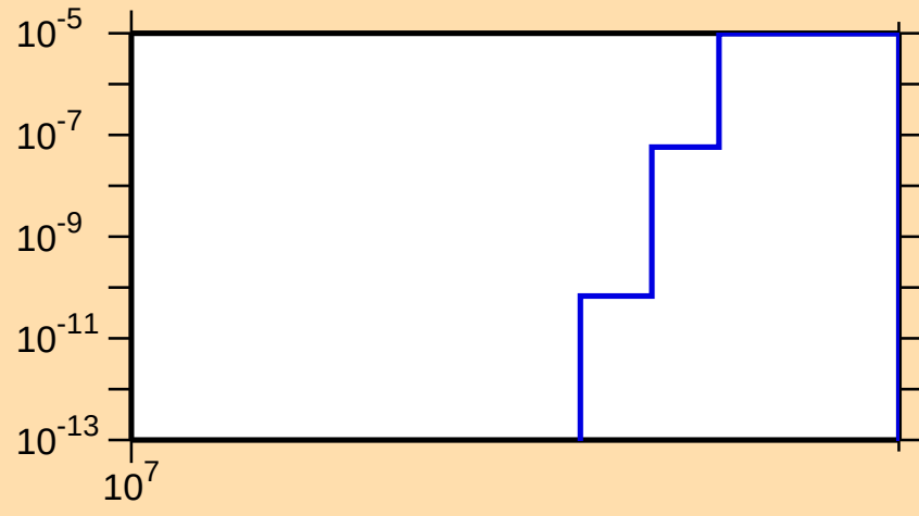
\sigma vs. E for ^{77}\text{Kr}(n,\text{nd})
