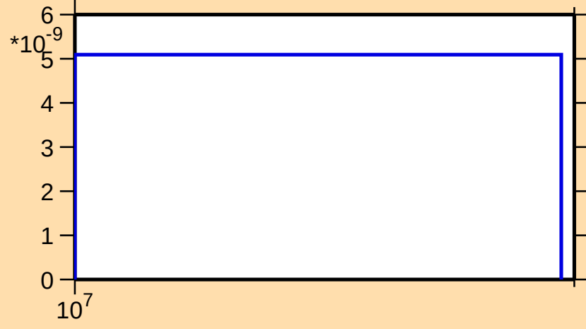
\sigma vs. E for ^{77}\text{Kr}(n,\text{pt})
