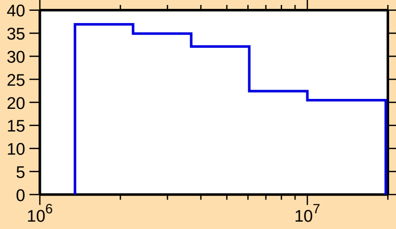
\Delta\sigma/\sigma vs. E for ^{77}\text{Kr}(\text{n},\text{inel.})
