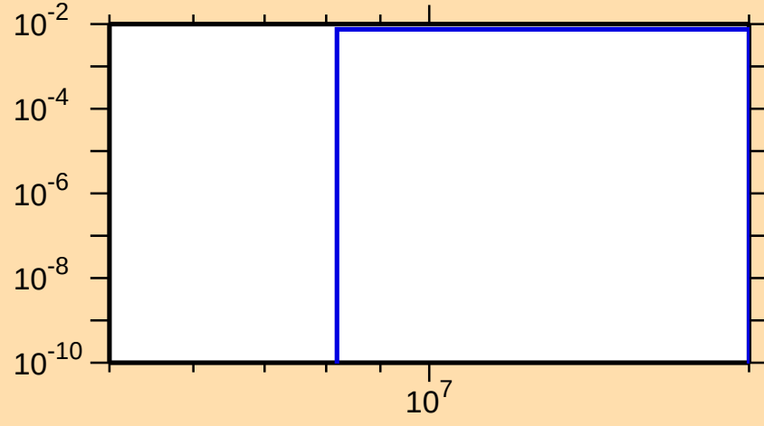
\sigma vs. E for ^{77}\text{Kr}(n,n\alpha)
