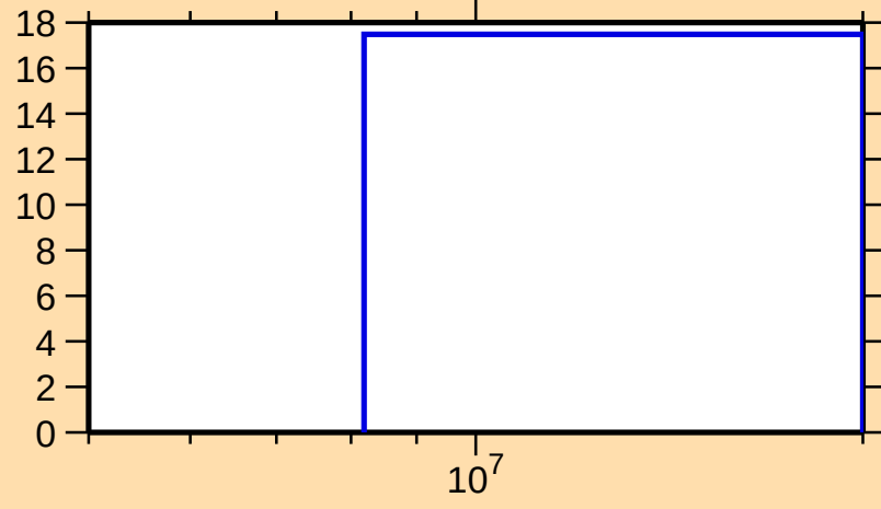
\Delta\sigma/\sigma vs. E for ^{77}\text{Kr}(n,\text{inel.})
