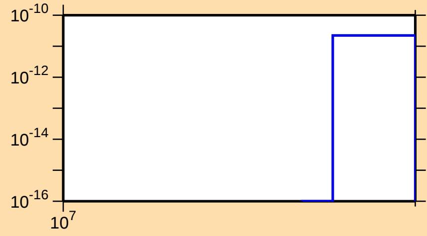
\sigma vs. E for ^{79}\text{Kr}(\text{mt } 34)
