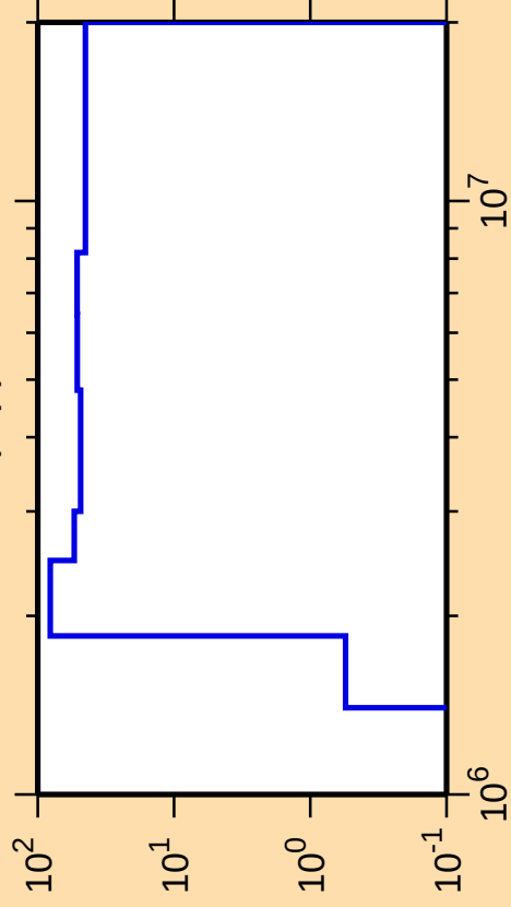
\Delta\sigma/\sigma vs. E for ^{80}\text{Kr}(n,p)
