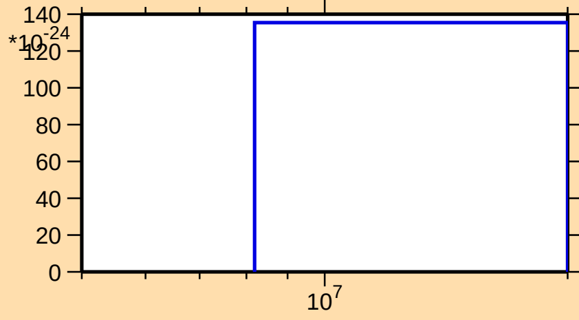
\sigma vs. E for ^{80}\text{Kr}(n,nt)
