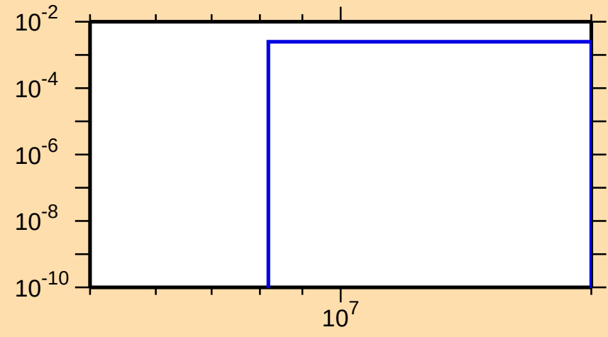
\sigma vs. E for ^{80}\text{Kr}(n,d)
