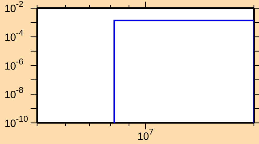
\sigma vs. E for ^{80}\text{Kr}(n,n\alpha)
