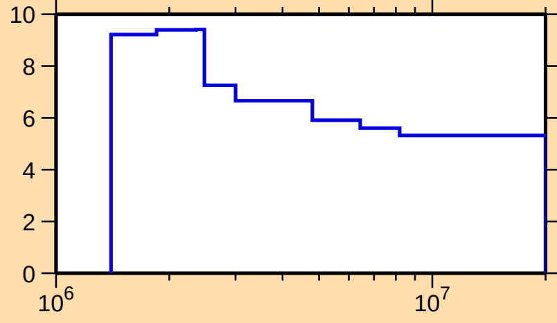
\Delta\sigma/\sigma vs. E for ^{80}\text{Kr}(n,\text{nonel.})
