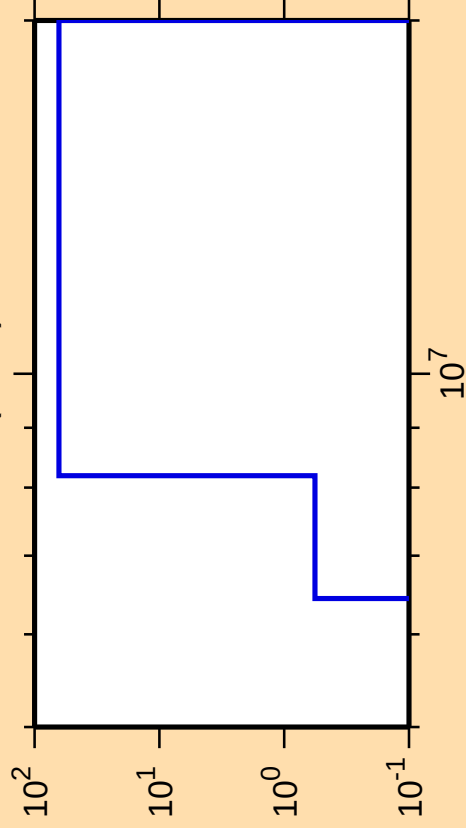
\Delta\sigma/\sigma vs. E for ^{80}\text{Kr}(n,n\alpha)
