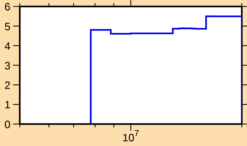
\Delta\sigma/\sigma vs. E for ^{81}\text{Kr}(n,\text{nonel.})
