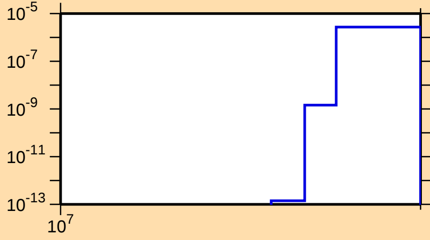
\sigma vs. E for ^{81}\text{Kr}(n,nd)
