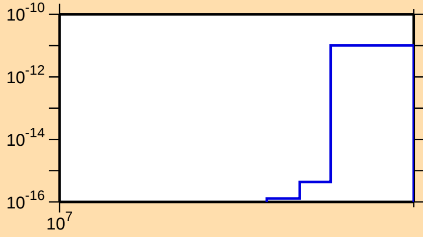
\sigma vs. E for ^{81}\text{Kr}(n,\text{pt})
