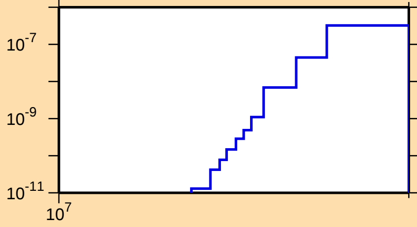
\sigma vs. E for ^{81}\text{Kr}(n,p\alpha)
