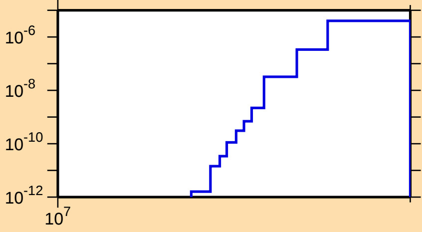
\sigma vs. E for ^{81}\text{Kr}(n,\text{He}3)
