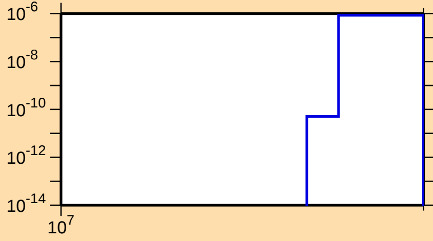
\sigma vs. E for ^{83}\text{Kr}(n,\text{nd})
