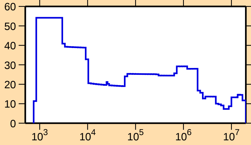
\Delta\sigma/\sigma vs. E for ^{83}\text{Kr}(\text{n,el.})
